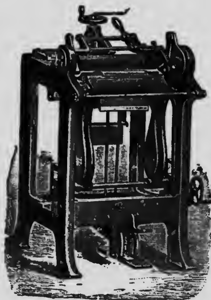
Fig. 41—Backing machine for large shops.
