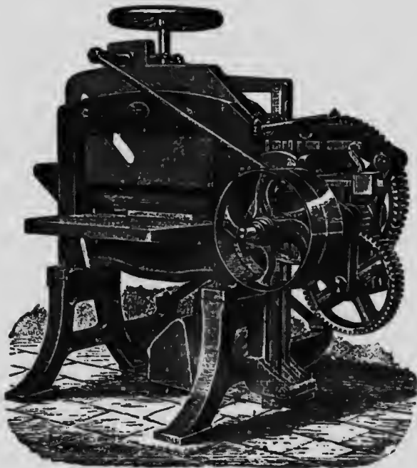
Fig. 35—Rotary guillotine.
