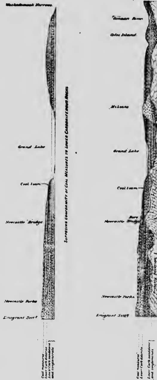
DIAGRAMATIC SECTIONS OF THE GRAND LAKE COAL BASIN, QUEENS COUNTY, N.B.
