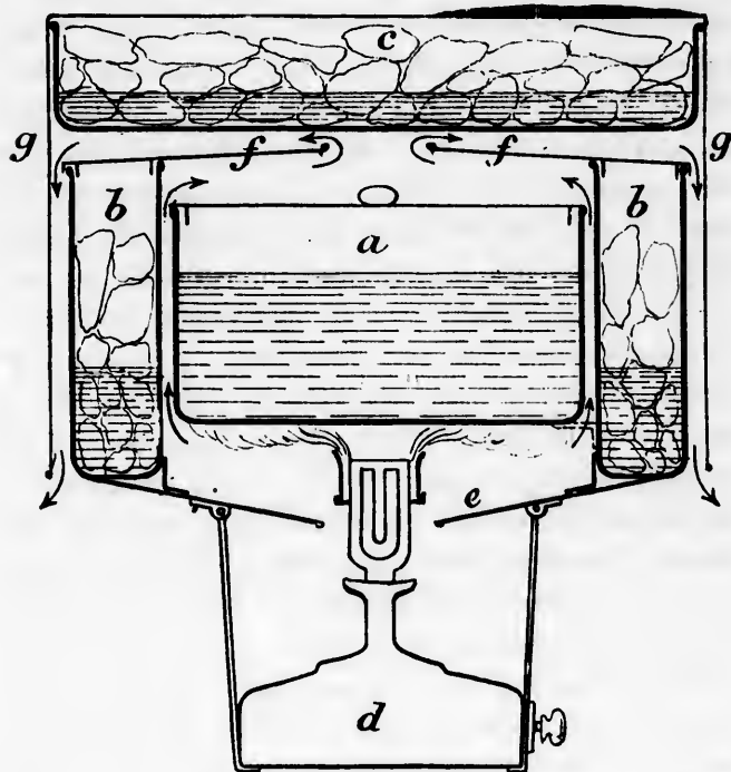
THE COOKING APPARATUS.
