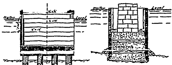
Fig. 71. Concrete-filled bottomless Caisson.
