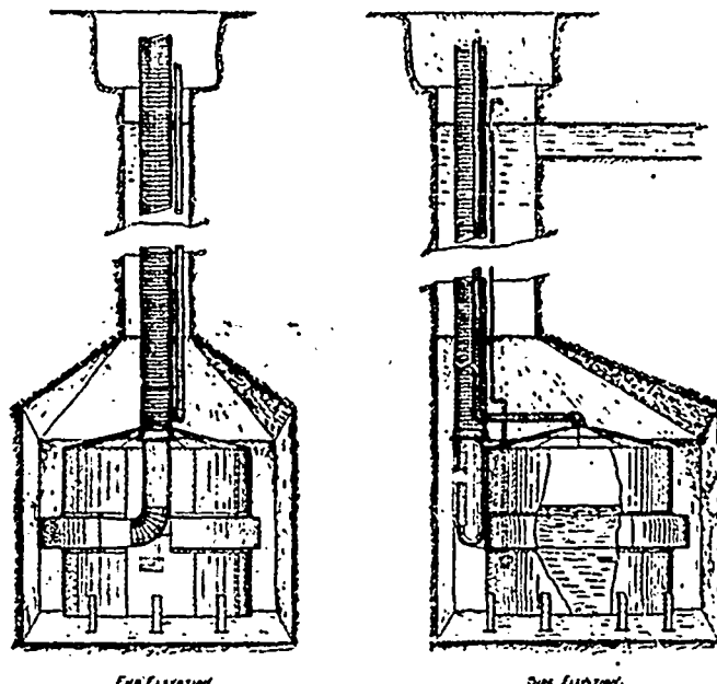
Taylor Hydraulic Air Compressor. KOOTENAI AIR SUPPLY CO. Coffee Creek, Ainsworth District, B.C. Size 18" x 12".
