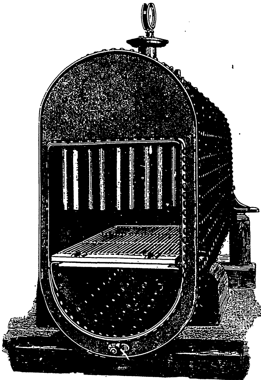
KINGSLEY BOILER—FRONT END VIEW OF NAKED BOILER READY FOR WATER TEST.
