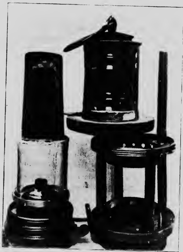
FIG. IX.—Gray's No. 2 Patent Safety Lamp for Deputies, Firemen or Miners. Showing gas-testing tube in position. Lead lock. Gives a particularly good light. Illuminant—paraffine or minerai colza.
