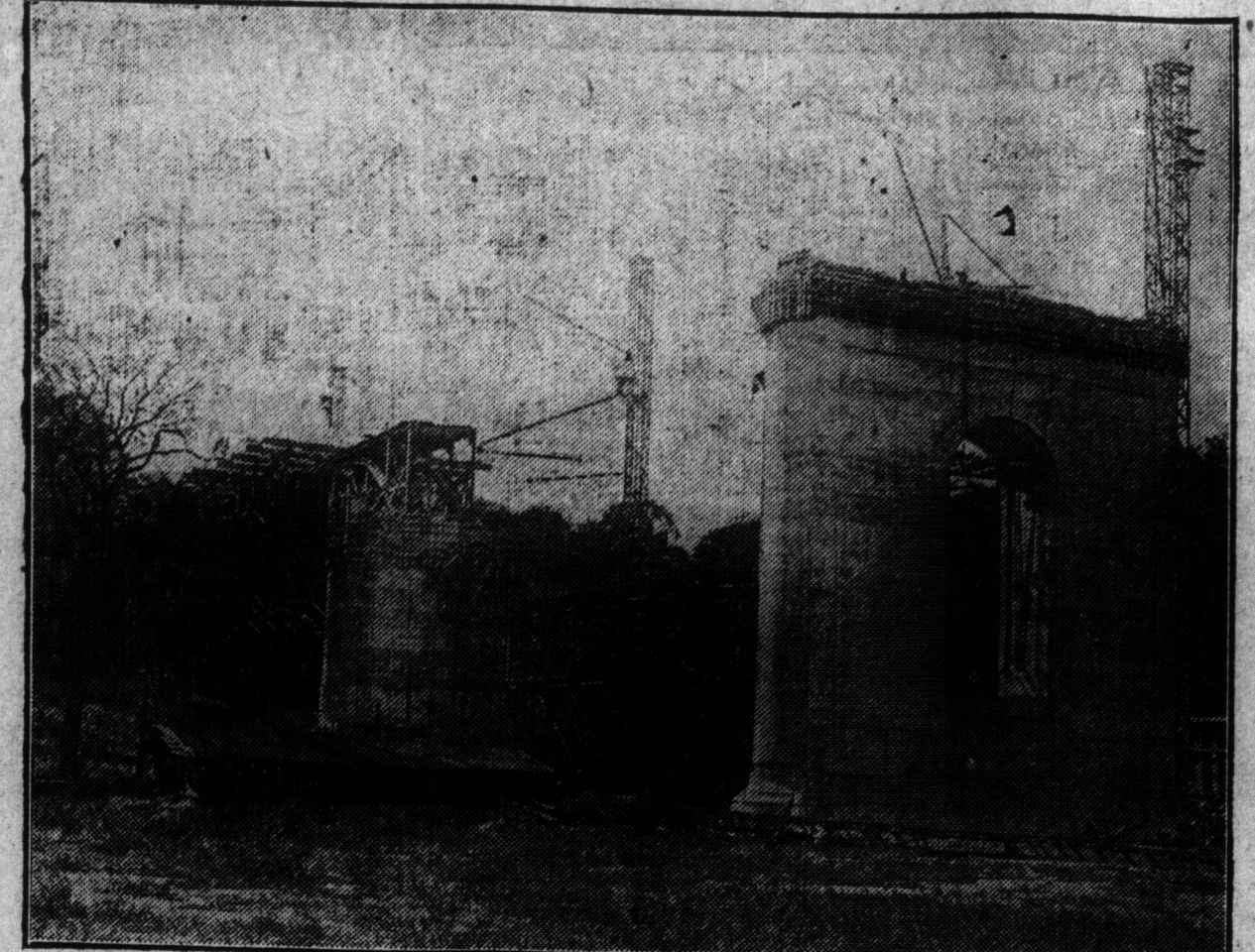
Bloor street viaduct looking west from the east side of the river and showing the cement pier that will carry the west end of the arch over the bridge. This pier will be carried up by the railroads immediately under the street surface of the bridge. The picture also shows the second arch, partially finished, and the steel arch and its supports about completed. The road grade landing is at the extreme back.
