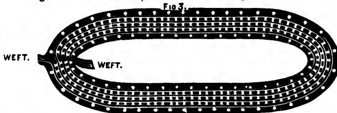
Figure 3.—Shows the position of the Filling in a Four-ply Hose.
