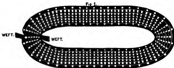
Figure 1.—Shows the position of the Filling in a Six-ply Hose.
