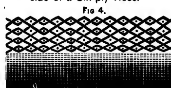
Figure 4.—Sectional view of a Four-ply Hose.
