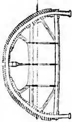
Fig. 3. Transverse section amidships.
