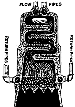
SECTIONAL VIEW.
