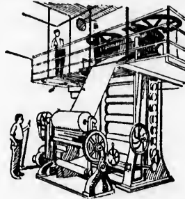
SUPER CALENDERING.
