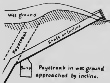
Fig 31. Section.
