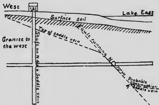
Fig 44. Problem No 4. Section along saddle at Mooseland.
