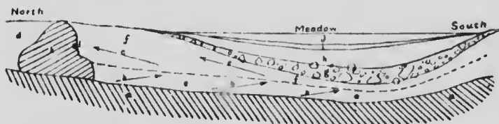
Fig 41. Problem No 2 Section of drift at West Caledonia Showing reversed drift transportation
