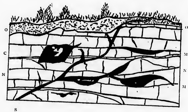
The above section shows a common occurrence of Galena Veins. oo—Surface Clay. NN—Limestone. M—main bodies of ore. c—a Pocket. s—the Lode.
