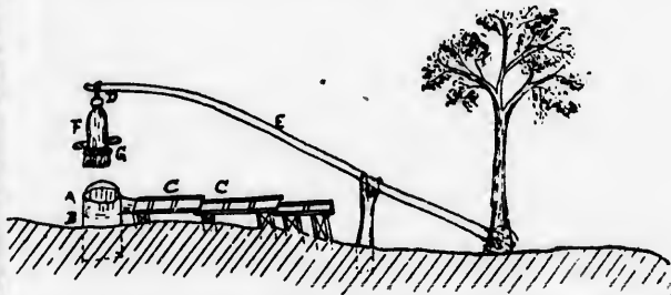
A.—Cushion bars. B.—Hollowed block. C.—Sluices. D.—Chain-hook. E.—Spring pole. F.—Dolly. G.—Iron shoe.
