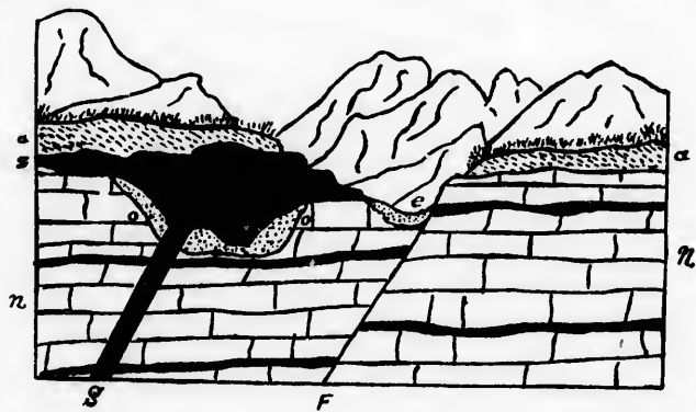
This section shows an old river bed covered by a trap overflow, which forced the river to take a new course, along the line of a "fault." A A —Earth. E —New Channel. O O —covered gold-bearing gravel. N N —The formation. F —Fault. S S —Trap overflow.
