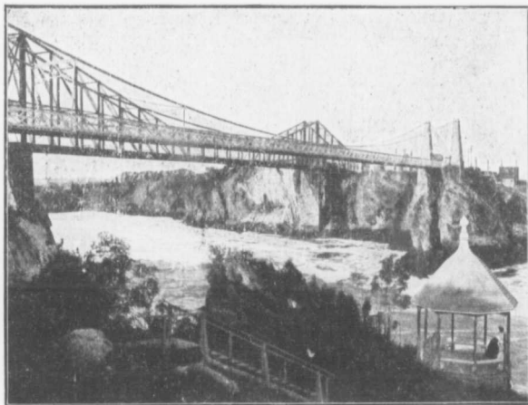
ST. JOHN BRIDGE AND FALLS AT LOW WATER. (From a photograph by Isaac Erb & Son, St. John.)
