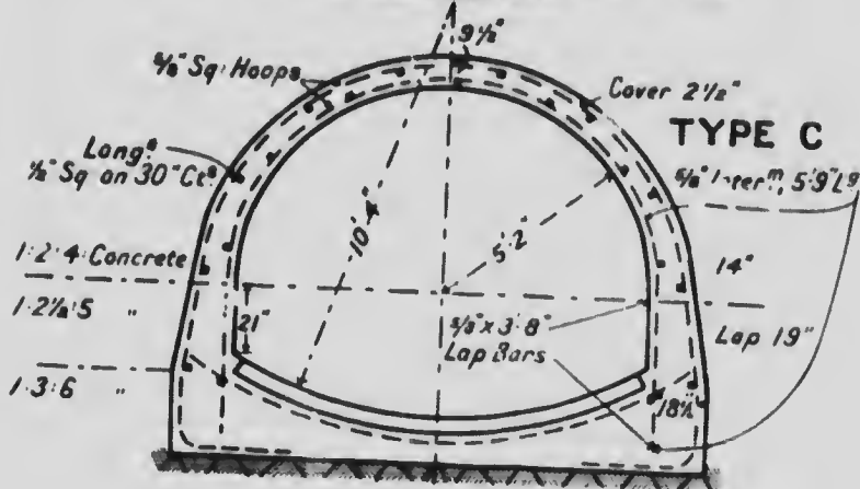
TYPICAL SECTIONS BALACLAVA ST. TRUNK SEWER VANCOUVER, B. C.
