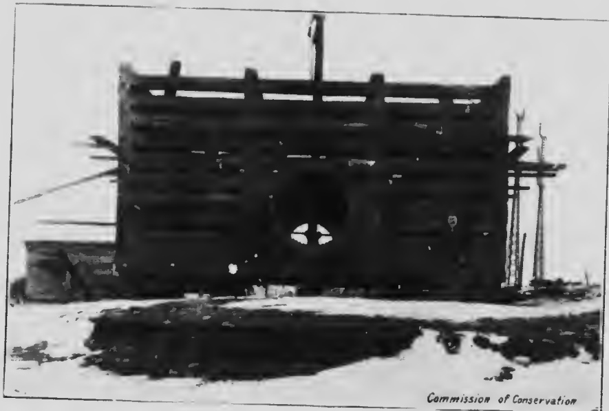
Hamilton Water-works - Crib at the End of 48 inch Intake Pipe
