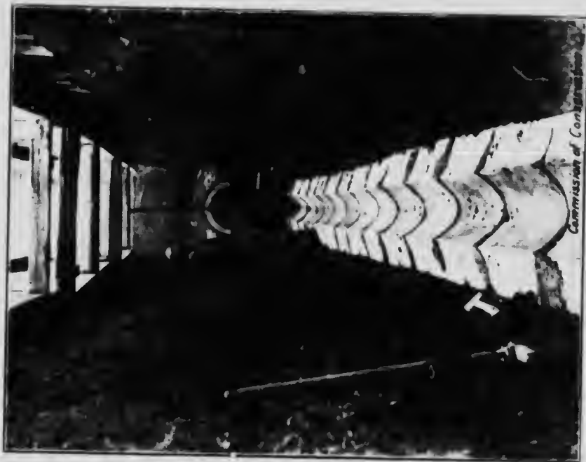
Brandon Sewerage System — Laying 48 inch x 32 inch Elliptical Concrete Sewer
