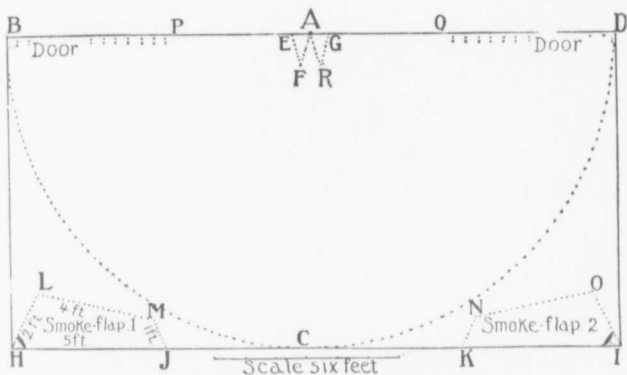
CUT I.—PATTERN FOR A SIMPLE 10-FOOT TEEPEE
