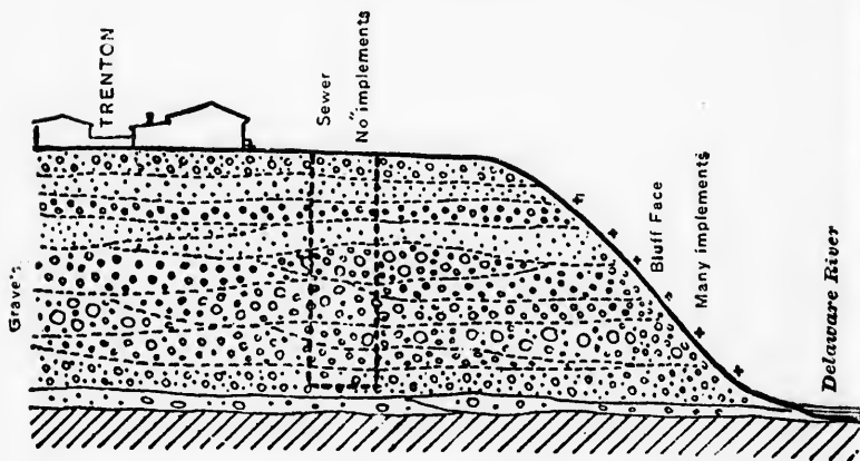
SECTION AT TRENTON, ON THE DELAWARE, SHOWING THE RELATION OF THE STONE IMPLEMENTS TO THE GLACIAL (?) GRAVELS (after Holmes)
