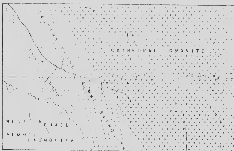
FIGURE 32.—Map showing relations of the Cathedral and Rimmell batholiths and the Ashnola gabbro. The Younger Phase of the Cathedral granite is shown by stippling. The remarkably straight contact line of the Cathedral granite lies sensibly parallel to the gneissic banding in the Rimmell batholith, Eastern Phase. Scale:—1 : 118,000.
