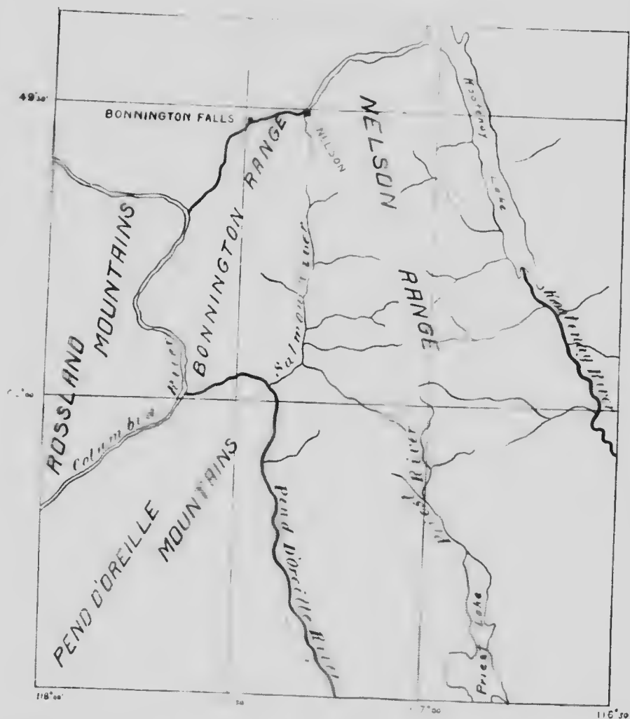
FIGURE 3.—Diagrammatic notes showing sub-division of the Selkirk Mountain System at the Forty-ninth Parallel.
