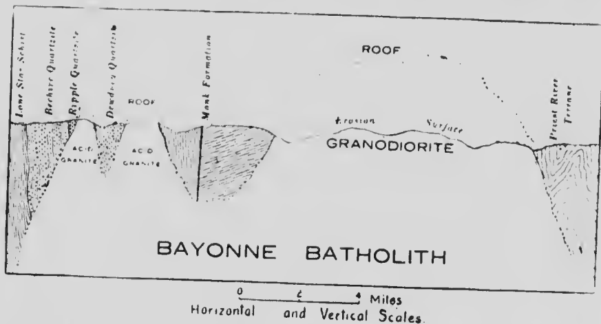
FIGURE 22.—Diagrammatic section showing relation of the summit stocks of Nelson Range to the Bayonne batholith.
