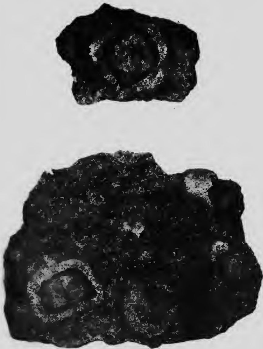
Specimens of nodule-bearing peridotite from forty-foot dike cutting schistose rocks of Basic Complex. The nodules are granular aggregates of olivine, regularly surrounded with kelyphitic shells, as shown. Two-thirds natural size.
