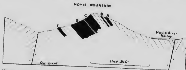
Figure 14—Section of Moyie mountain and the Moyie sills, along the International Boundary line. Sills in solid black. Bedding planes of the quartzite and fault planes shown.
