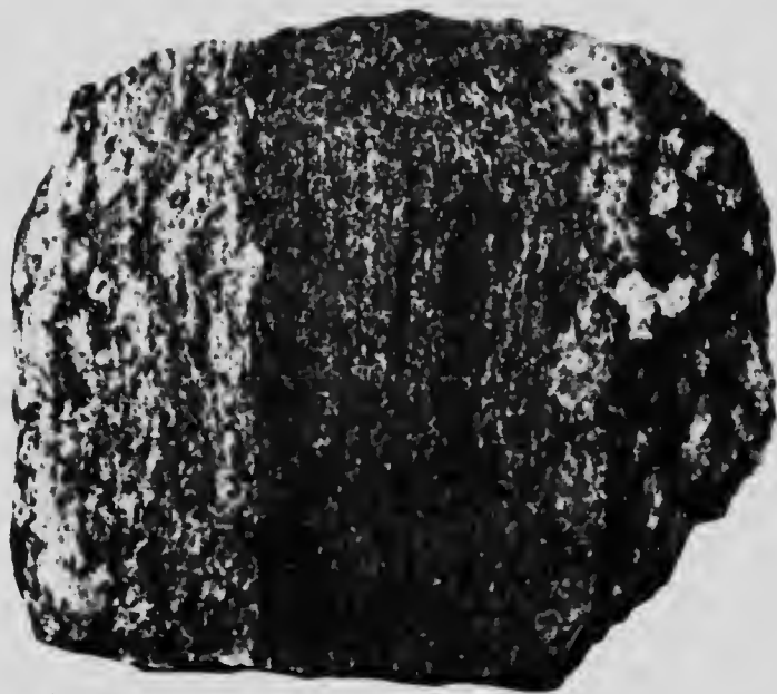
Sheared phase of the Rykert granite, showing concentration of the ferrous elements of the rock (middle zone). Natural size.
