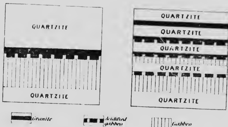
Figure 16. Diagram illustrating the hypothesis that the partially differentiated syntectic magmas of a thick sill may break through the roof and form, at stratigraphically higher horizons, several thinner sills differing in composition among themselves. Some later differentiation in the derived sills is assumed. The original sill is shown in the drawing on the left; the derived sills and the remnant of the original sill are shown in the drawing on the right. The channels (dikes) connecting the sills are not indicated.
