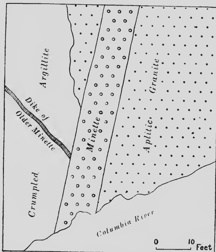
FIGURE 23. Map showing relations of Pond D'Oreille argillite, aplitic granite, and two dikes of minette, just south of Boundary line on the shore of Columbia River.
