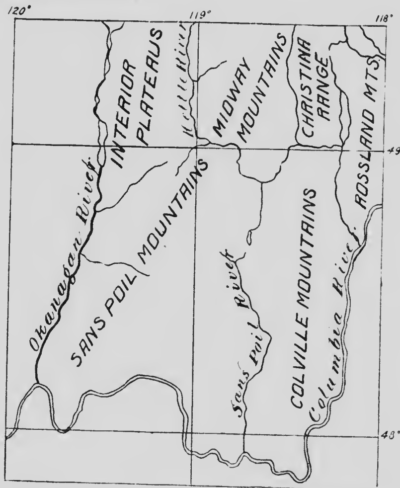
FIGURE 4. Diagrammatic map showing subdivision of the Columbia Mountain System at the Forty-ninth Parallel.
