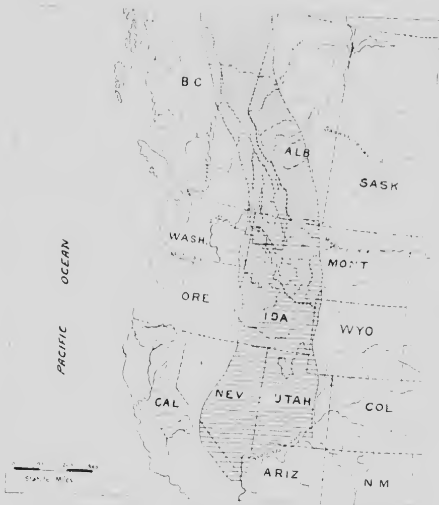
Figure 12. Diagrammatic map showing approximate position of the Rocky Mountain Geosynclinal province in the Beltian, Lower Cambrian, and lower Middle Cambrian pre-Flathead phases.
