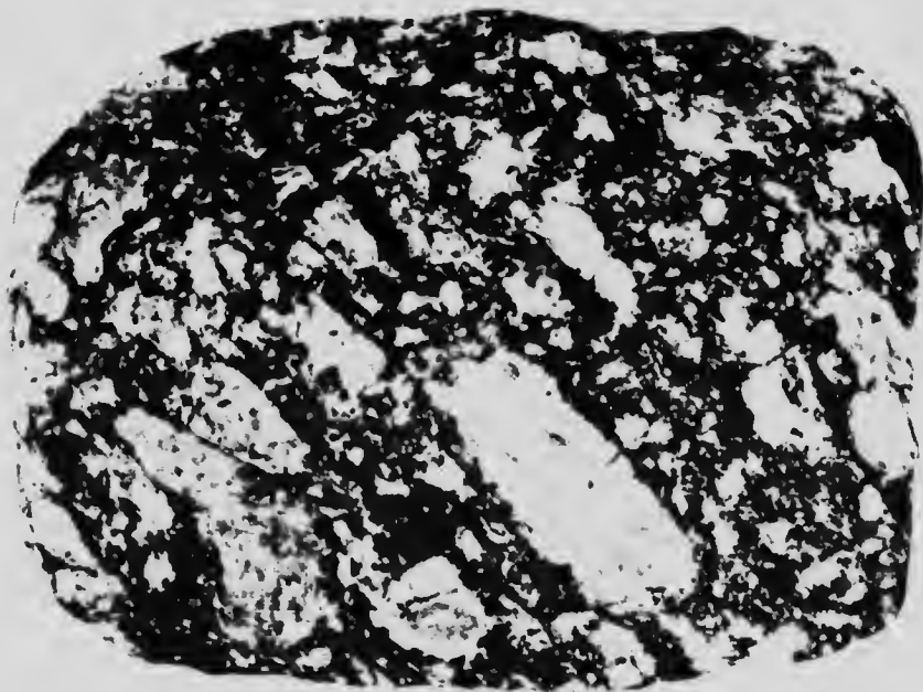
Massive phase of the Rykert granite, showing large phenocrysts of alkali feldspar. 20a—vol. II, p. 284.
