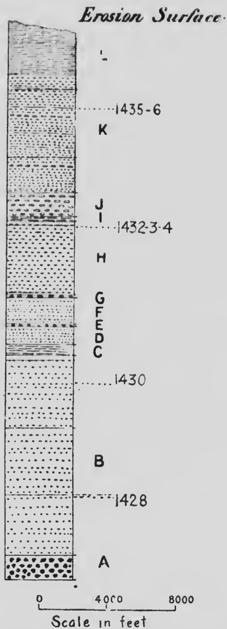
FIGURE 34. Columnar section of the Pasayten Series, including the Pasayten Volcanic formation (member A). Approximate horizons of fossils indicated by collection numbers.
