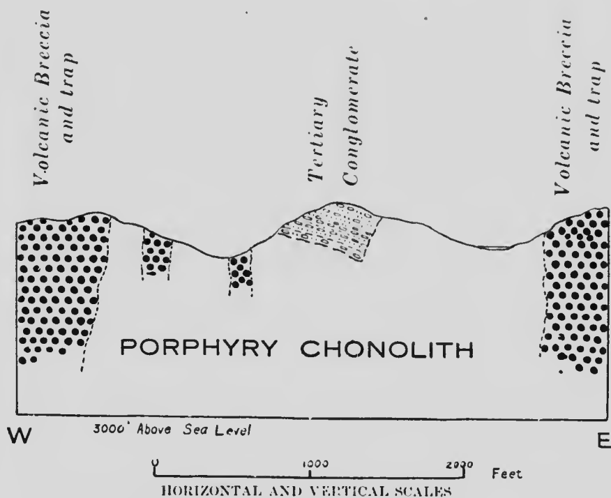
FIGURE 24.—Section of syenite porphyry chonolith, satellite to Coryell batholith.
