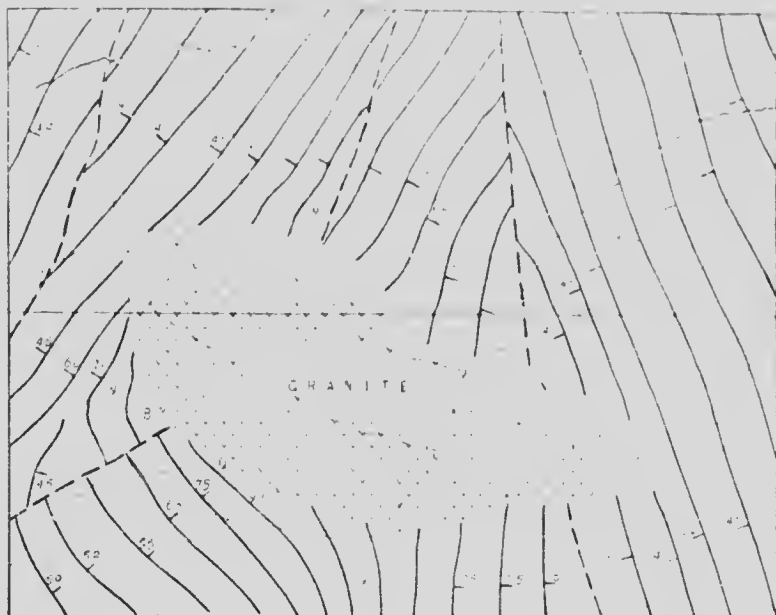
FIGURE 35. Map showing relation of Peak stock to the deformed Pasayton formation. Strike at point nearest shown; faults in broken lines. Scale: 1:115,000.
