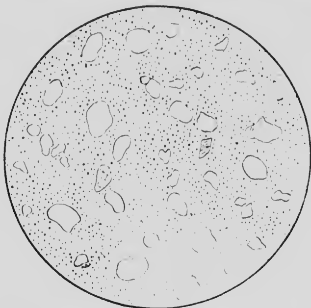
FIGURE 8. Diagrammatic drawing from thin section of typical sandy dolomite of the Altyn formation. Round (wind-blown?) grains of quartz (clear white) and much less abundant microperthitic feldspar (transverse lines) drawn to scale. The dots represent, on the same scale, the size of the extremely minute carbonate granules composing the matrix of the rock. Diameter of circle 4.5 mm.
