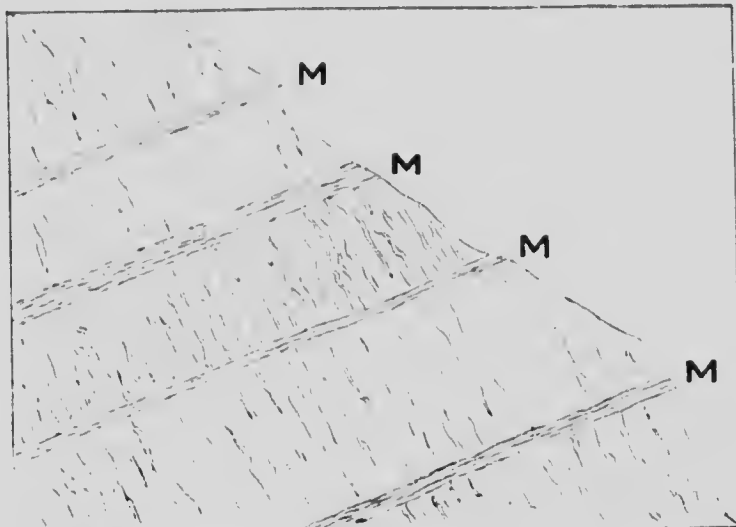
FIGURE 9.—Section showing common phase of the polar tooth structure in the Siyeh formation. The calcitic segregations are lenticular and stand perpendicular to the plane of stratification, as shown by the metargillitic interbeds (M). The middle layer of limestone is two feet thick. Locality, north fork of the Yellowstone River.
