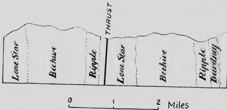
Figure 17.—East-west section on ridge north of Lost Creek, Nelson Range; showing duplication of beds by thrust, the plane of which has been rotated.
