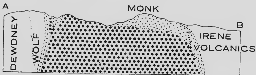
FIGURE 21.—Section along line A-B of figure 20, on the same scale; illustrating explanation of great breadth of metamorphic aureole southeast of larger granite stock. Apophysal dikes in roof of stock not shown.
