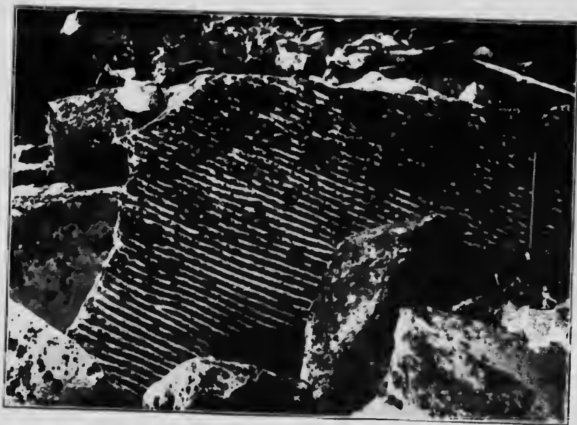
Ripple-marks in Ripple-quartzite; negatives (casts). Same locality and scale. 25a—vol. ii—p. 154.
