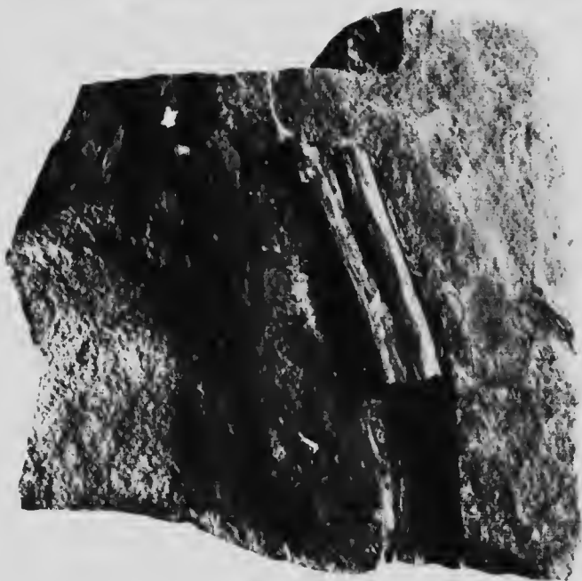
Fossil plants in the Kettle River sandstone. In upper view, east of a pine cone of Tertiary age. Natural size.
