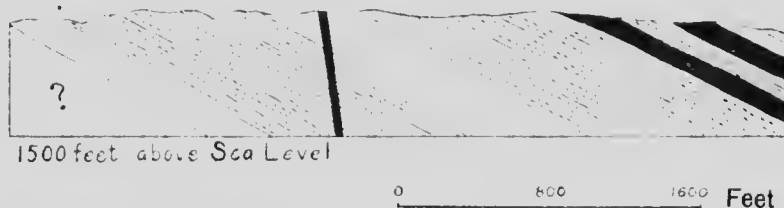
FIGURE 25.—Section northeast of bridge over Kettle River, six miles above Midway.
