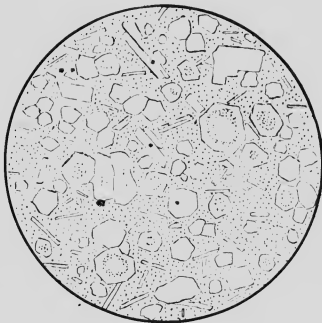
FIGURE 26. —Partly diagrammatic drawing from thin section of ground-mass of "shackanite" (neither phenocrysts nor the rare pyroxene granules of ground-mass shown). The roundish, often polygonal crystals are analcite, with and without minute inclusions. The rectangular, trapezohedral, and lath-shaped crystals are alkali feldspar. Magnetite grains represented in actual proportion. All these crystals lie in a matrix of brown glass and serpentine (dotted). Diameter of circle, 1 mm.
