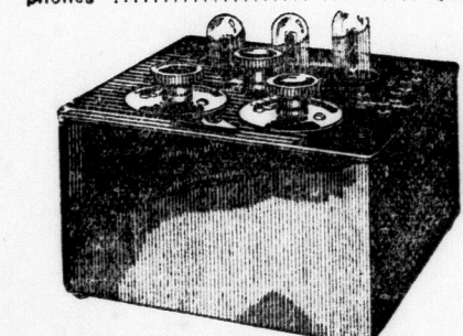
CANADIAN GENERAL ELECTRIC MODEL 93 Equipped with two U. X. 199 radiotrons, one U. X. 120-power tube and phones $89.00
