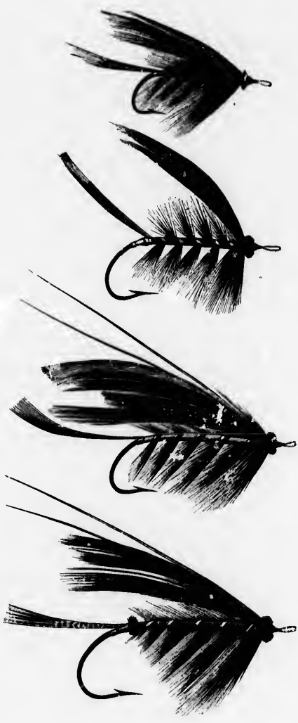
SALMON FLIES.
