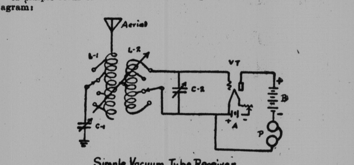
Simple Vacuum Tube Receiver
