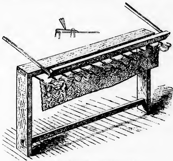
THE FIRST KNITTING MACHINE. LEE.
