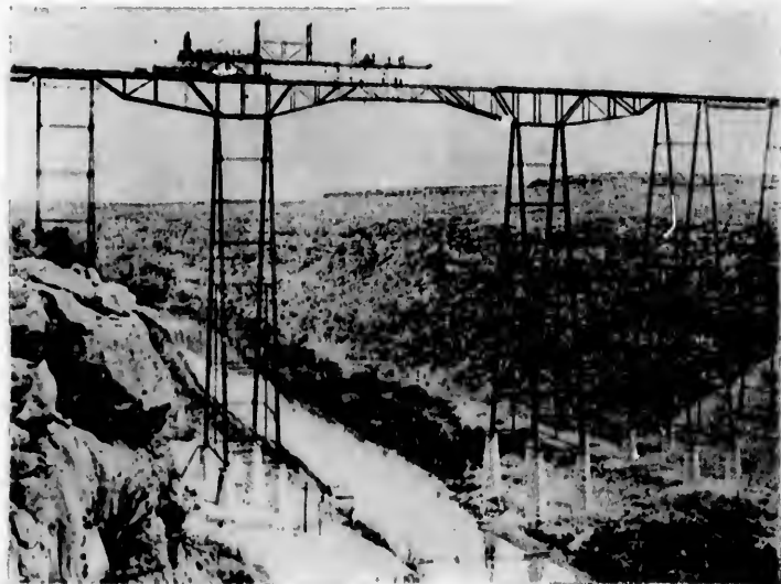
PECOS RIVER VIADUCT.
