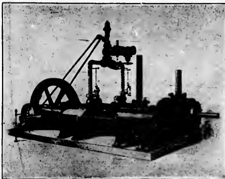
INGERSOLL-SERGEANT DUPLEX STEAM-ACTUATED AIR COMPRESSOR.
