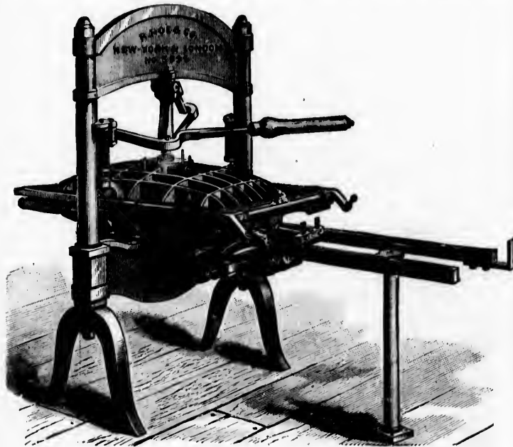
WASHINGTON HAND PRESS.
