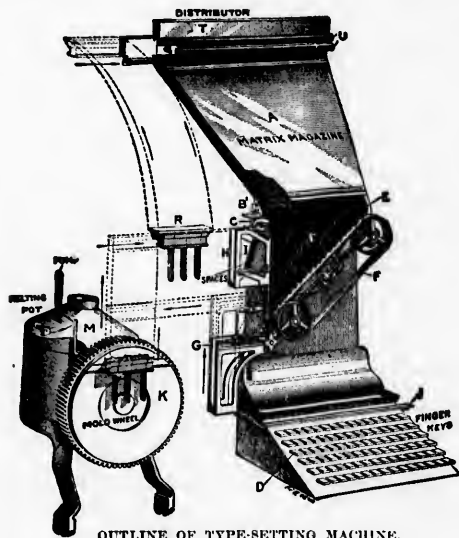
OUTLINE OF TYPE-SETTING MACHINE.
