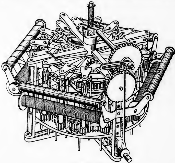
CIRCULAR LOOM.
