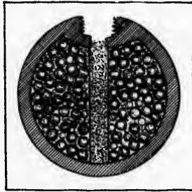
OLD STYLE SHRAPNEL.
