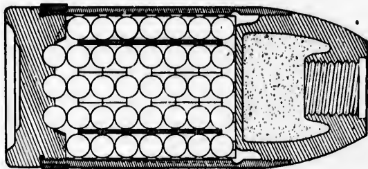
MODERN SHRAPNEL.
