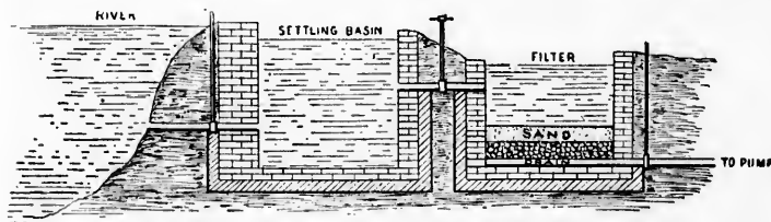
SAND FILTER BED.
