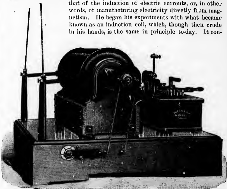
INDUCTION COIL.
