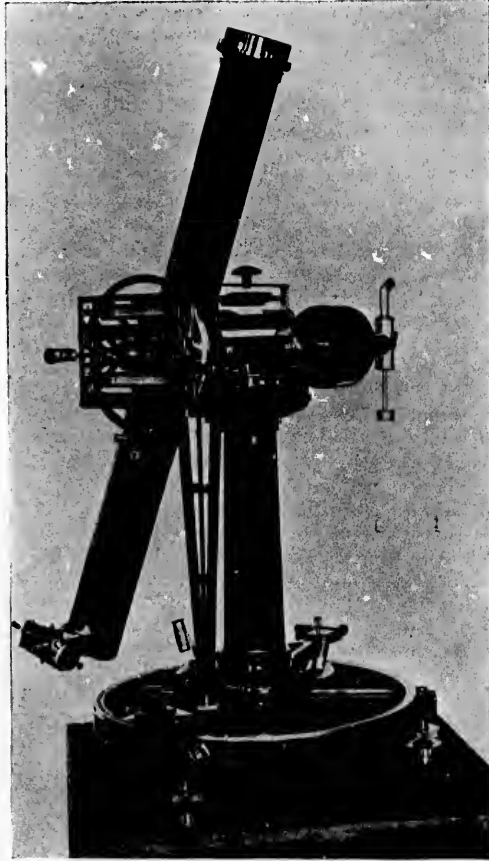
ZENITH TELESCOPE.
