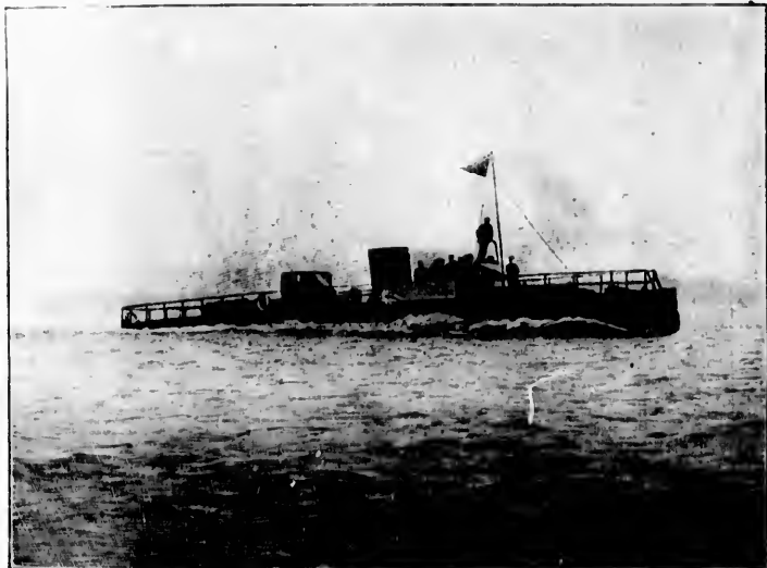
THE TURBINIA.
