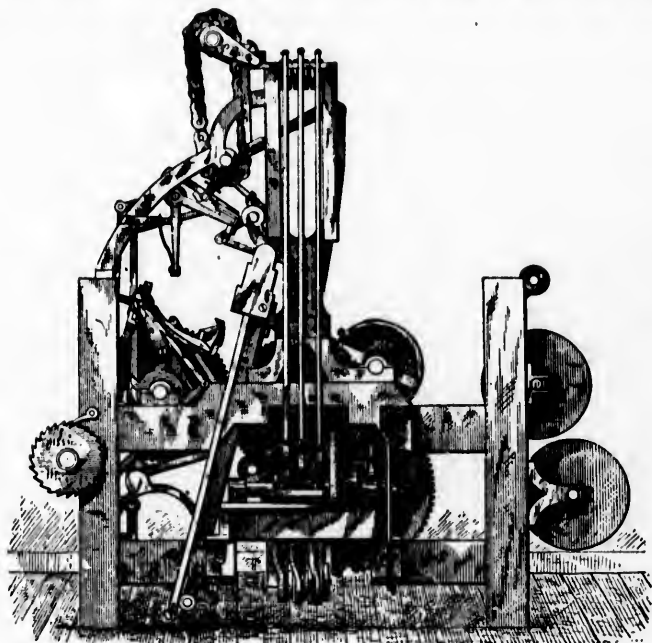
SMITH AND SKINNER LOOM FOR MOQUETTE CARPETS.
