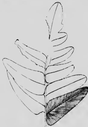
FIG. 15. Osmunda macrophylla n. sp. Extremity of a frond from the Red Deer River. x 11. 9197-9
