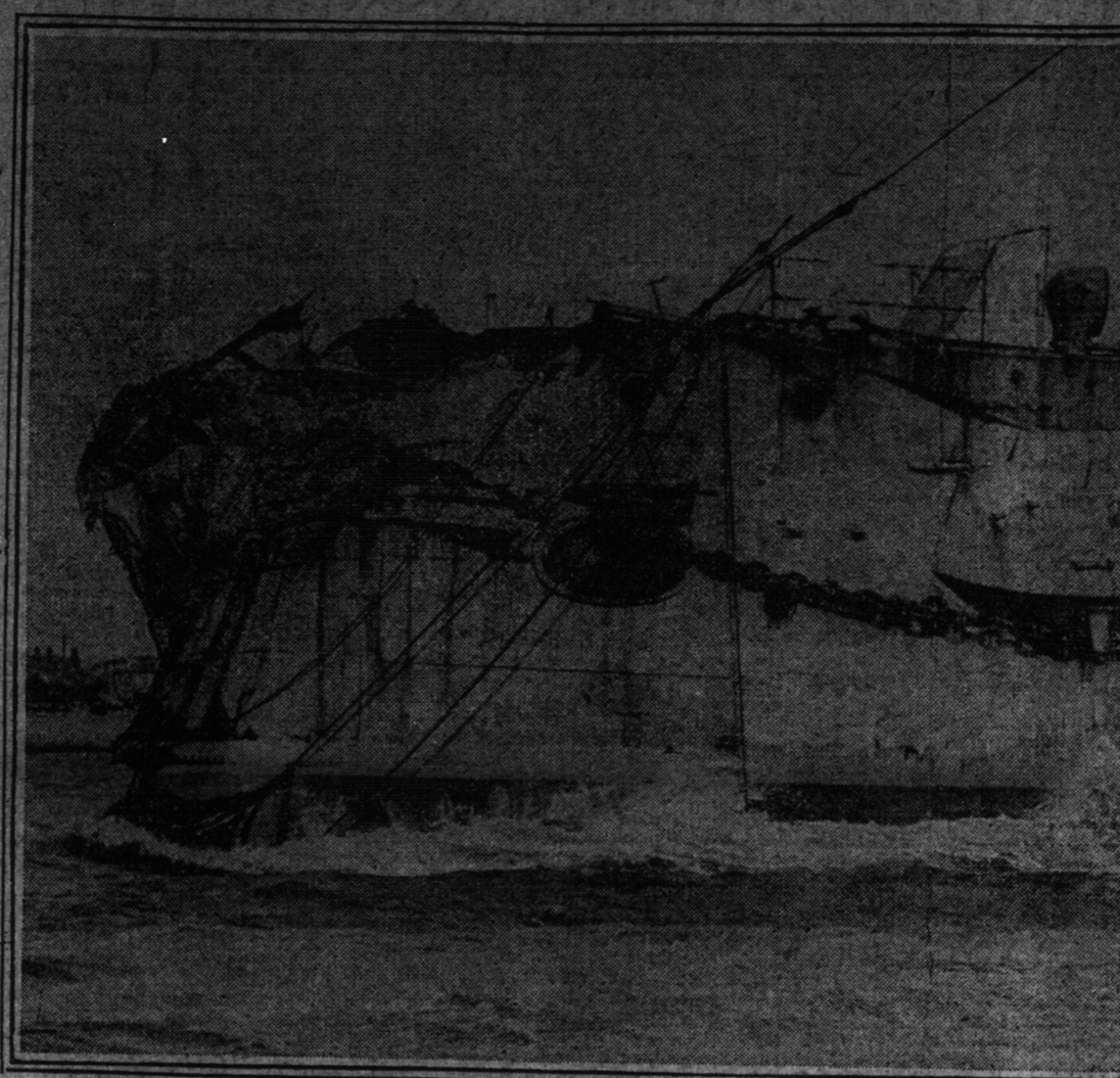
CLOSE VIEW OF THE HAWKE, SHOWING HER DAMAGED BOWS, AND A COLLISION MAT IN POSITION. This photograph conveys a very good idea of the damage done to the British cruiser Hawke when that vessel rammed into the White Star line steamship Olympic recently in Osborne Bay, Isle of Wight.
