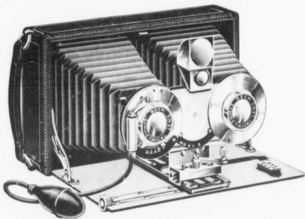
Fig. 7—THE STEREO "RALLI"
