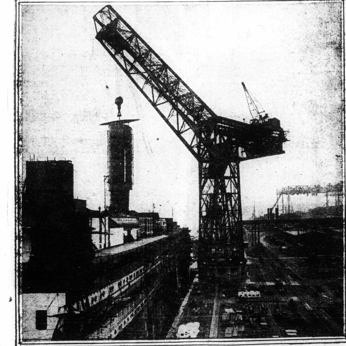
PLACING THE WATERLAND'S FUNNELS IN POSITION AT HAMBURG. The funnel is seen suspended from one of the big cranes which have been adopted by many engineering yards in other countries. The Waterland, Germany's giant transatlantic liner, is now being completed at Hamburg and will take her place in the express service on June 5. The huge ship has a tonnage of 55,000, which is 3,000 tons in excess of her older sister ship, the Imperator. She is 897 feet long, 95 feet broad and 62 feet in depth.
