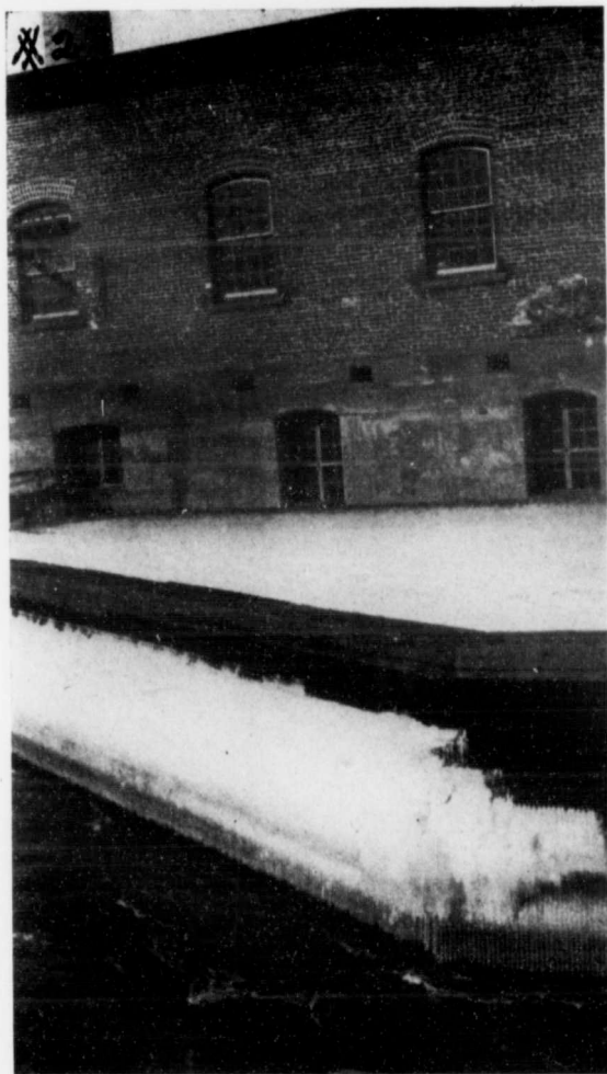
FIG. 33 —Iron Rack which has been submerged during the night previous by adhering Frazil stopping the flow. Large masses are seen still clinging to the bars.
