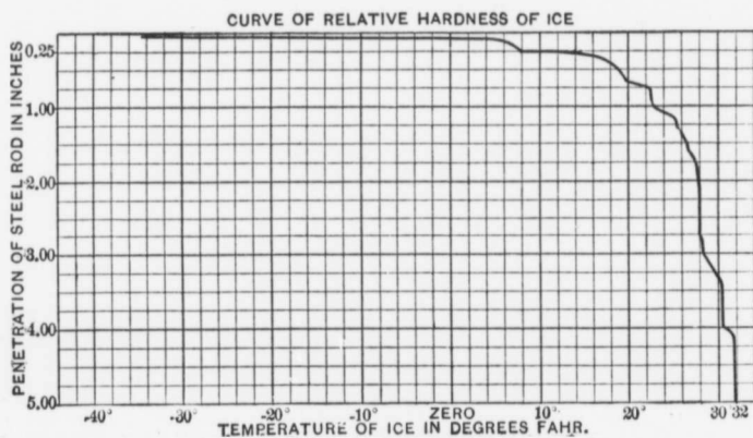
FIG. 14.—Andrews's Curve for Relative Hardness of Ice at Different Temperatures.
