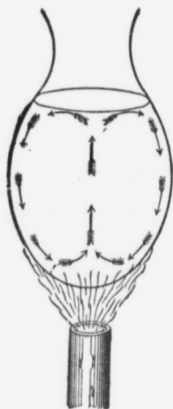
FIG. 5.—Convection Currents in Water.
