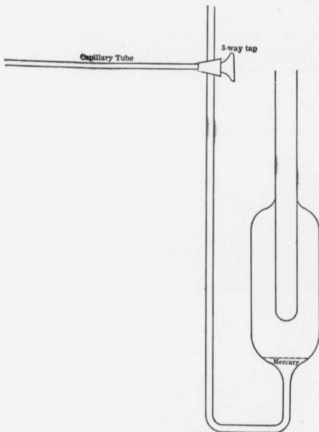
FIG. 15.—Bunsen Ice-calorimeter.
