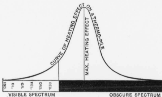
FIG. 1.—Distribution of Heat in Spectrum.
