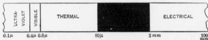
FIG. 3.—Diagram of Ether Spectrum.
