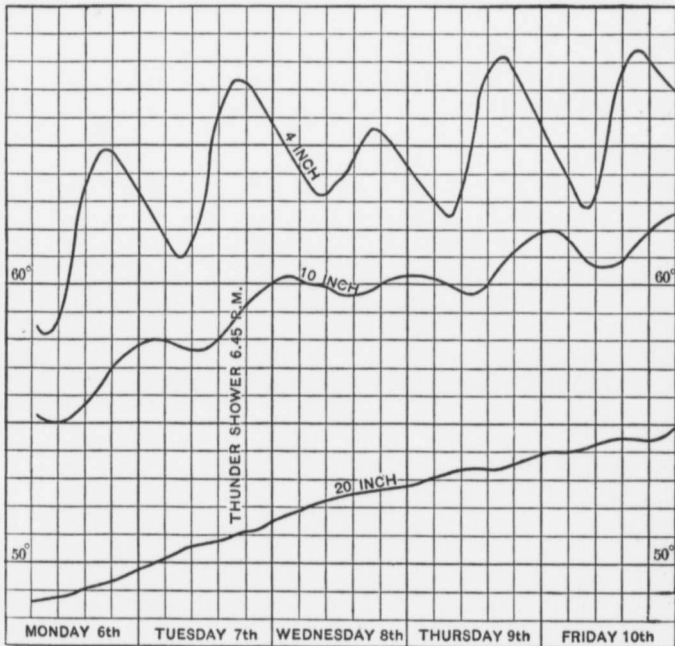
FIG. 4.—Diurnal Waves of Heat in the Earth. Callendar and McLeod.
