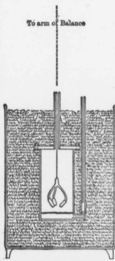
FIG. 11.—Apparatus of Barnes and Cooke.
