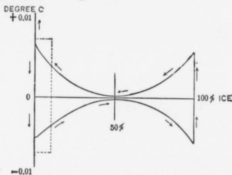
FIG. 30.—Freezing-point Diagram.
