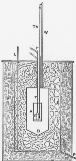
FIG. 12.—Calorimeter used by A. W. Smith for Latent Heat of Water.
