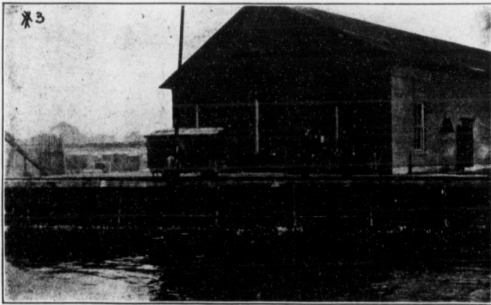
FIG. 34.—Horizontal steam-pipes shown in place on the same iron rack previous to lagging. Electric scraper shown for removing frazil from the rack.
