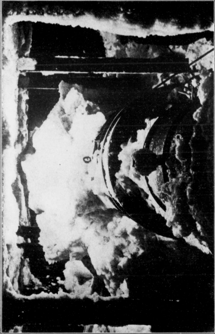
FIG. 36.—Penstock or Wheel-house which has been blocked by frazil drawn in through the racks. The ice has been mostly removed previous to the photograph.
