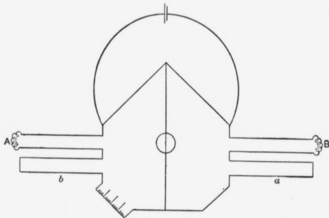
FIG. 24.—Diagram of Differential Platinum Thermometer Connections.
