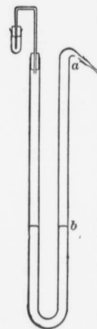
FIG. 9.—Bunsen's Dilatometer.
