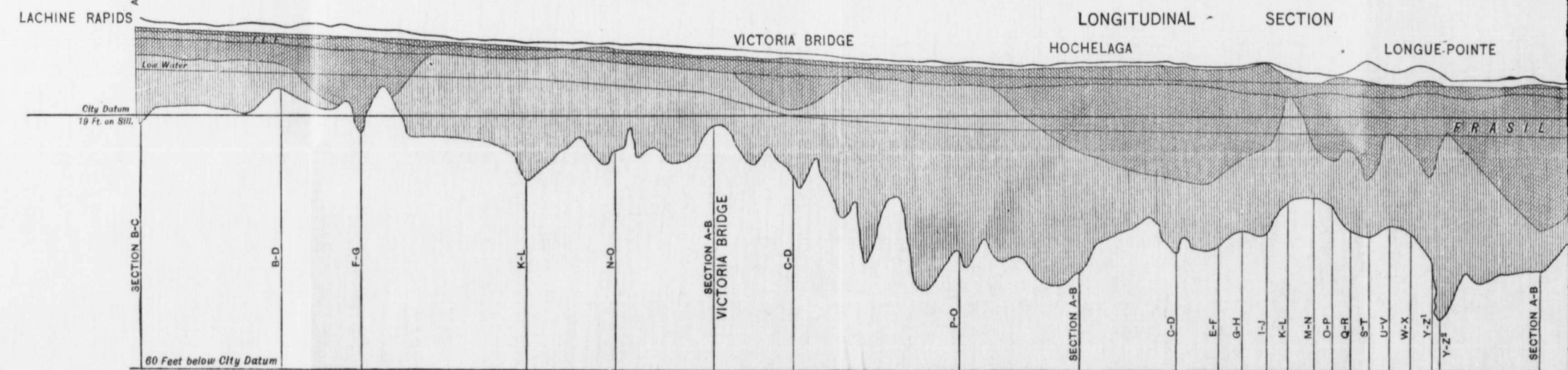
FIG. 40. Four sections of the St. Lawrence River in winter, showing the accumulations of frazil-ice under the surface-ice.
