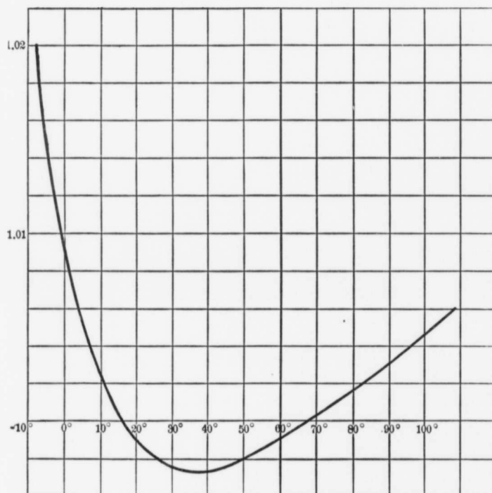
FIG. 13.—Variation of the Specific Heat of Water. (Barnes.)
