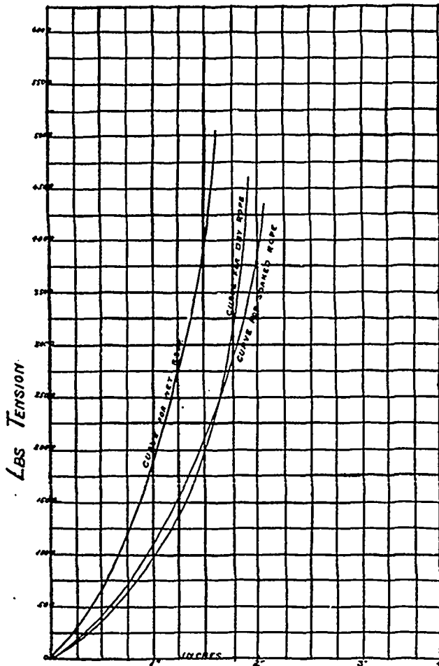
DIAGRAM SHOWING RELATION OF EXTENSION TO LOAD FOR MANILLA AND HEMP (TARRED) ROPE
