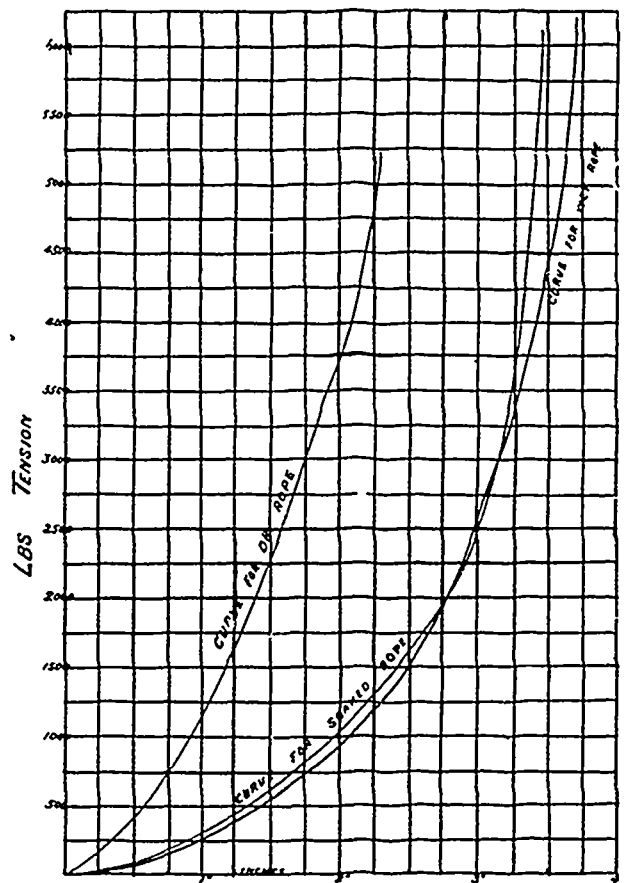
DIAGRAM SHOWING RELATION OF EXTENSION TO LOAD FOR MANILLA AND HEMP (UNTARRED) ROPE
