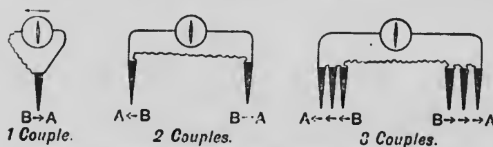
Fig. 178. - Scheme of thermo-electric couples. (After Waller.)
