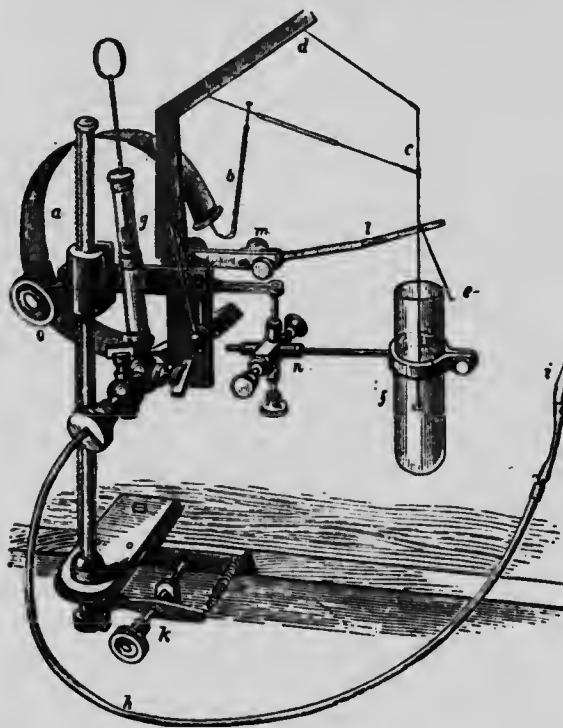
Fig. 279.—Fick's Kymograph, improved by Hering (after McKendrick). a , hollow spring filled with alcohol, bearing lever arrangement b, d, c , to which is attached the marker e ; the rod c passes downwards into the tube f , containing castor oil, which offers resistance to the oscillations of c ; g , syringe for filling the leaden tube h with saturated sulphate of sodium solution, and to apply sufficient pressure as to prevent the blood from passing into the tube h at i , the cannula inserted into the vessel; l , abscissa-marker, which can be applied to the moving surface by turning the screw m ; k , screw for adjusting the whole apparatus to the moving surface; o , screw for elevating or depressing the Kymograph by a rack-and-pinion movement; n , screw for adjusting the position of the tube f .
