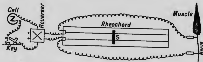
Fig. 193.—Arrangement of apparatus for demonstrating Pfüger's law.
