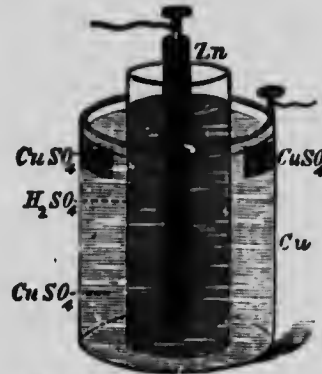
Fig. 133.—Diagram of a Daniell's battery.
