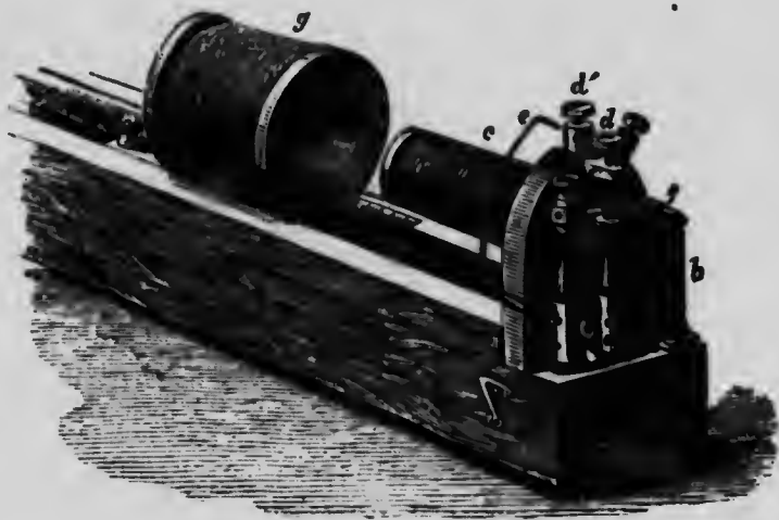
Fig. 137.—Du Bois Reymond's induction coil.
