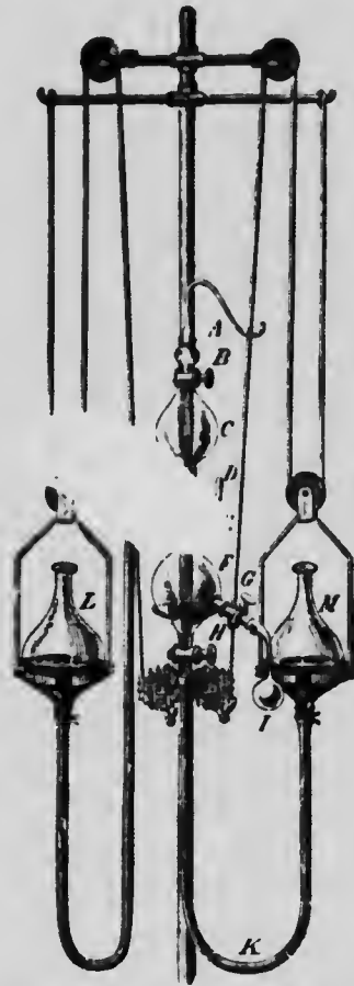
Fig. 333.—Ludwig's mercurial pump.
