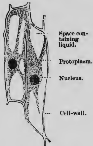
Fig. 1.—Vegetable cells.
