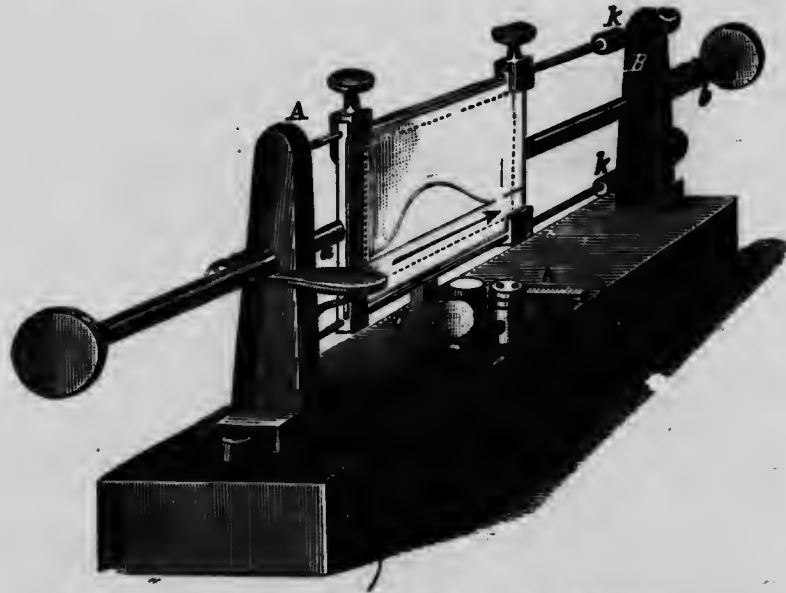
Fig. 142.—Du Bois Reymond's spring myograph. (M'Kendrick.)
