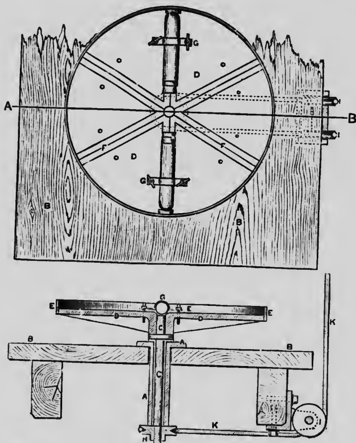
Fig. 341.—Plan and section of centrifugal machine. A, an iron socket secured to top of table B; C, a steel spindle carrying the turntable D and turning freely in A; E, a flange round turntable D; F F, shallow grooves on face of D in which the test tubes are fixed by clamps G G; H, a pulley fixed to end of spindle C and turned by the cord K; I I are two guide pulleys for cord K. The upper part of the figure is a surface view of the rotating turntable. (Gamble.)
