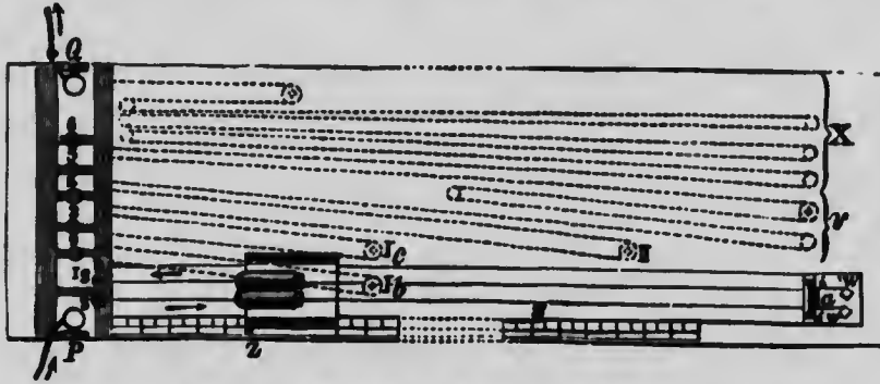
FIG. 187.—Poggendorf's rheochord. (M'Kendrick.)
