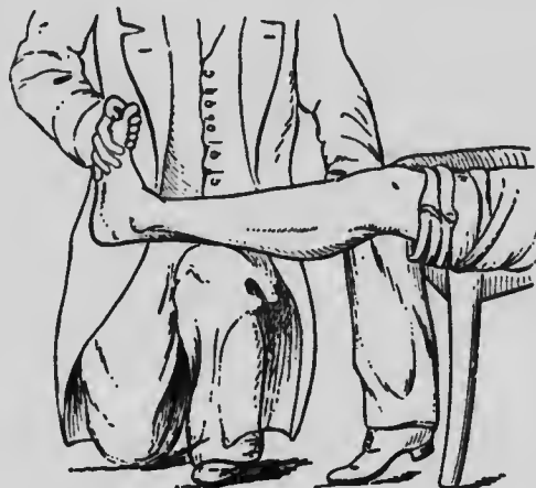
Fig. 491.—Ankle-clonus. (Gowers.)
