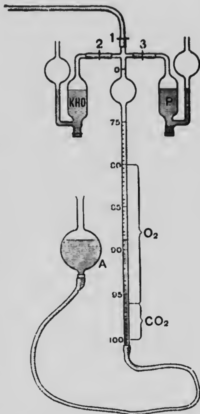
Fig. 335.—Waller's apparatus for gas analysis.
