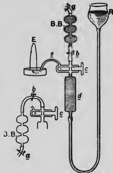
Fig. 334.—L. Hill's air-pump.
