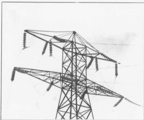
DETAILS OF A TRANSPOSITION TOWER
