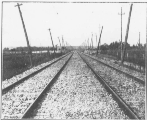
DOUBLE TRACK PERMANENT WAY—HAMILTON RADIAL ELECTRIC RAILWAY
