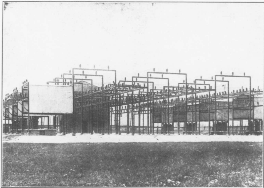
THE OPEN AIR SWITCHING STATION, BARTONVILLE Hamilton Cataract Power, Light and Traction Company, Limited "Dominion Power and Transmission Company."
