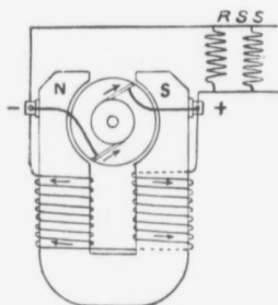
SHUNT WOUND DYNAMO
