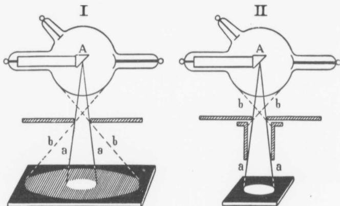
Fig. 40. Effect of Diaphragms.
