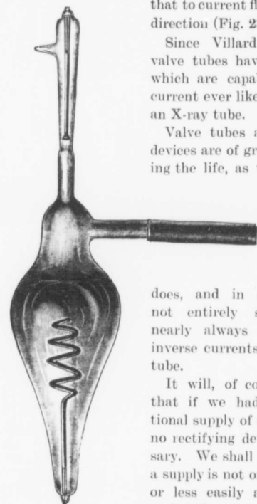
Fig. 23. Villard's Valve Tube.
