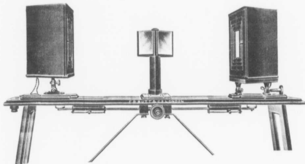
Fig. 48. Wheatstone's Stereoscope.
