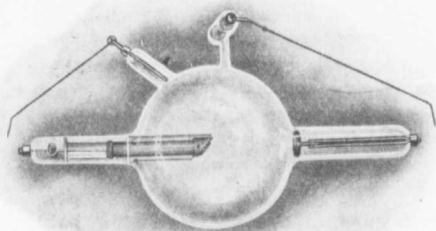
Fig. 14. Mica Regulator—in accessory bulb above.
