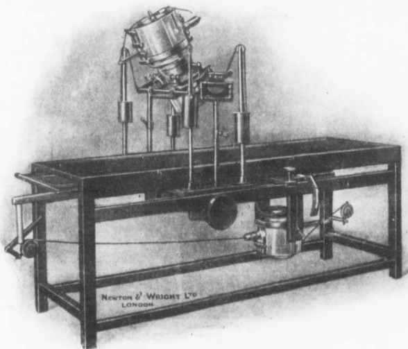
Fig. 71. Universal X-Ray Couch.
