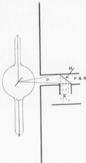
Fig. 72. Scheme for production of secondary rays.
