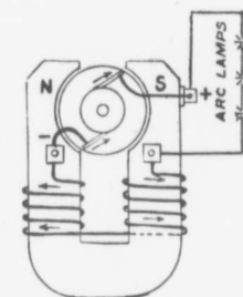
SERIES WOUND DYNAMO
