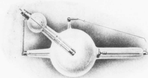
Fig. 16. Water-cooled Anti-Cathode.
