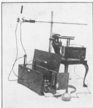
Fig. 28. Portable X-ray Outfit in use. A chair is used to clamp the tube-holder to.
