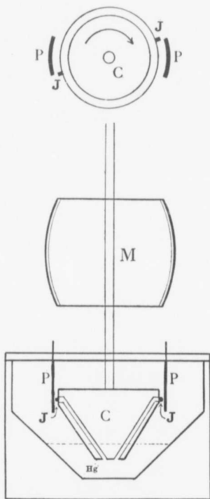
Fig. 31. Principle of Mercury Jet Interrupter.
