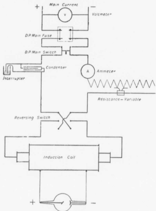
Fig. 36. Diagram of Induction Coil Circuits.
