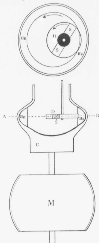
Fig. 34. Principle of Centrifugal Type of Mercury Interrupter. Above is shown a plan of section across the line A B.
