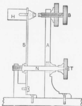
Fig. 30. App's Contact Breaker (from Wright's Induction Coil ).
