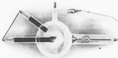
Fig. 17. Heavy Anode Tube.
