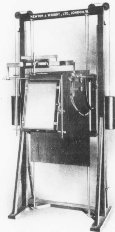
Fig. 60. Screening Stand.
