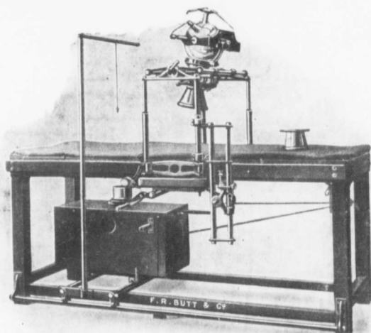
Fig. 39. A useful X-Ray Table for all classes of work.
