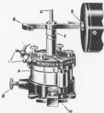
Fig. 33. Bécclère's Interrupter.
