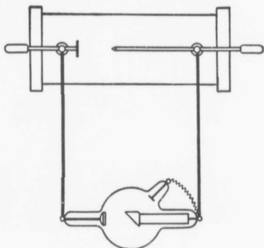
Fig. 13. Parallel Spark Gap.
