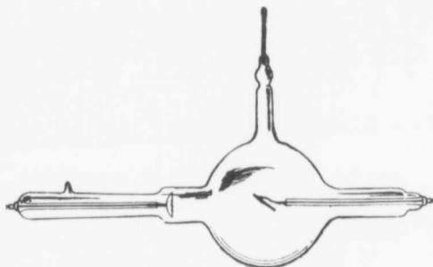
Fig. 15. Chabaud Tube with Osmo-regulator.
