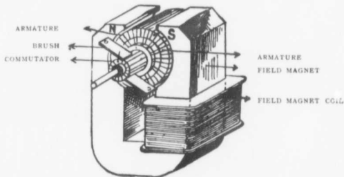
Fig. 5. Parts of a 2 Pole Dynamo.
