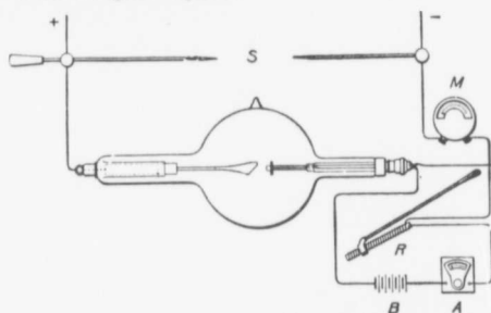
Fig. 21. Shewing arrangements for the Coolidge Tube.
