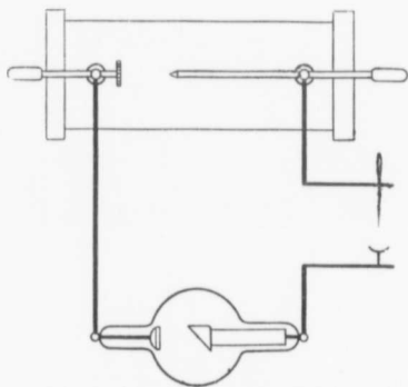
Fig. 22. A Series Spark-Gap between the anode and the coil to suppress any inverse current.
