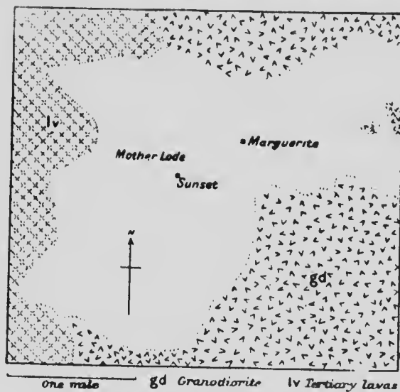
FIG. 2. Map showing distribution of granodiorite in the vicinity of the Mother Lode mine.
