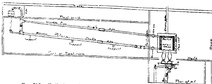
FIG. 712.—C. G. ATKINS' SYSTEM OF HEATING WITH KEROSENE LAMPS.
