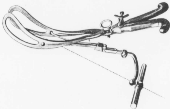
FIG. 149.—Tarnier's Axis-Traction Forceps.
