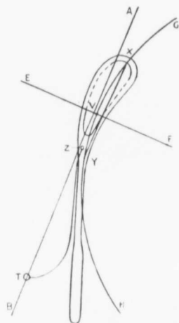
FIG. 153.—Mechanical Construction of Tarnier's Forceps. (Milne Murray.)
