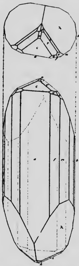
Figure 9. Diopside, colourless crystal from the Montreal chrome pit; idealized intermediate habit representing the average of a number of crystals, but with the length of the prism somewhat exaggerated.
