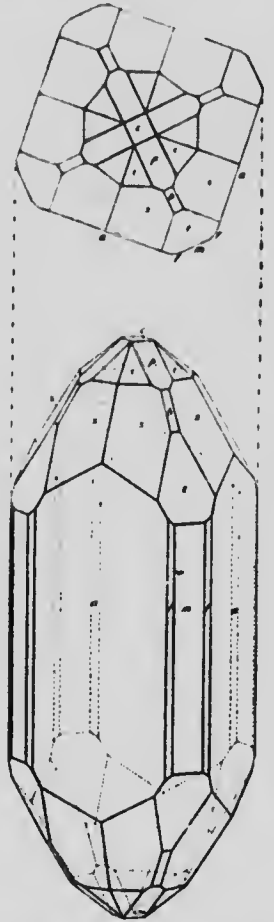
Figure 22. Vesuvianite from the Montreal chrome pit; average habit of the emerald-green crystals.
