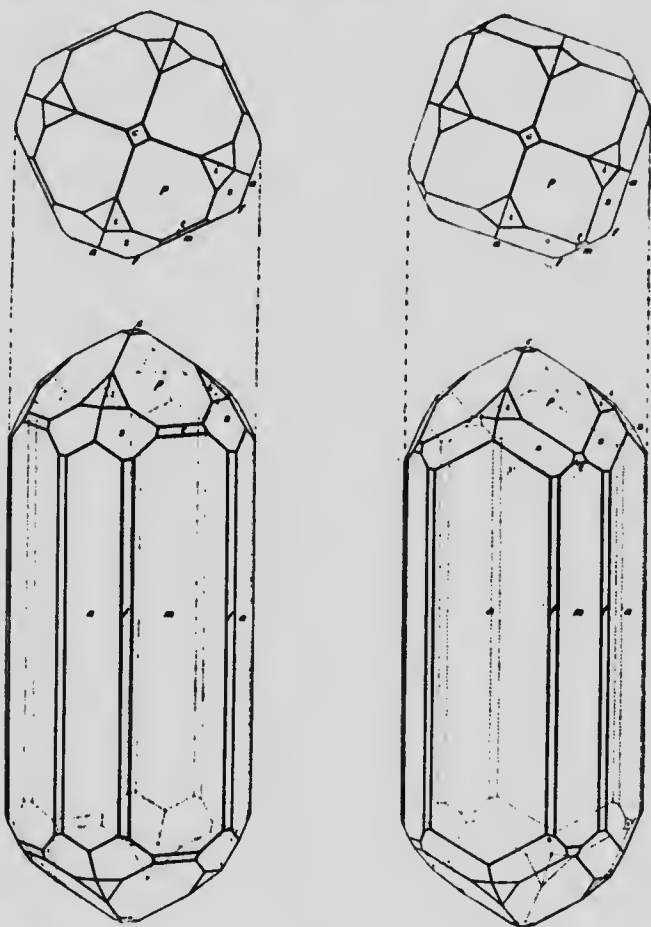
Figure 17. Vesuvianite, lilac crystal from the Montreal chrome pit; average habit when a(110) is larger than a(100) .
