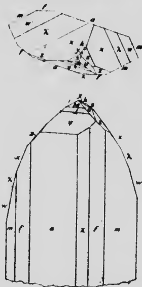
Figure 7. Diopside, colourless crystal from the Montreal chrome pit; illustrates the prominent development of the acute hemi-pyramid, \lambda(33\bar{1}) ; the crystal also exhibits the new forms Y and J .
