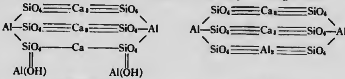
Constitutional formulæ of vesuvianite and garnet (after Clarke).
