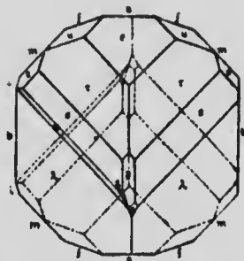
Figure 6. Diopside, colourless crystal from Montreal chrome pit; orthographic projection of one of the measured crystals, showing two of the new forms, s , (534) and r , (\bar{1}\bar{3}4\cdot10) .
