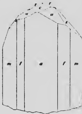
Figure 11. Diopside, colourless crystal from the Montreal chrome pit; crystal with somewhat flat termination, due to the equal development of the pyramidal forms \tau(\bar{1}12) , s(\bar{1}11) , x(\bar{2}21) , and \lambda(\bar{3}31) .
