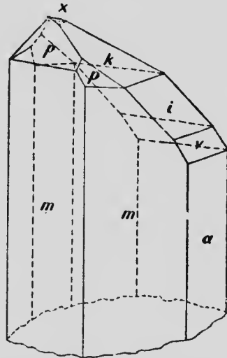
Figure 1. Aragonite from Montreal chrome pit, crystal twinned on m (110).
