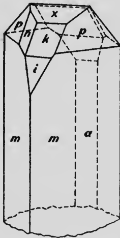
Figure 3. Aragonite from Montreal chrome pit, simple crystal with prominent development of the prism m (110).
