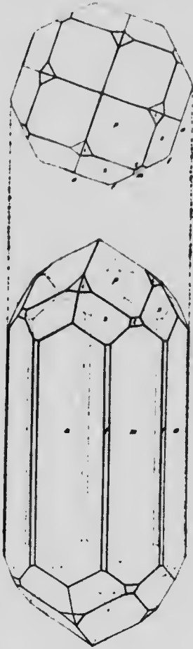
Figure 21. Vesuvianite from the Montreal chrome pit; average habit of the pale yellowish crystals.
