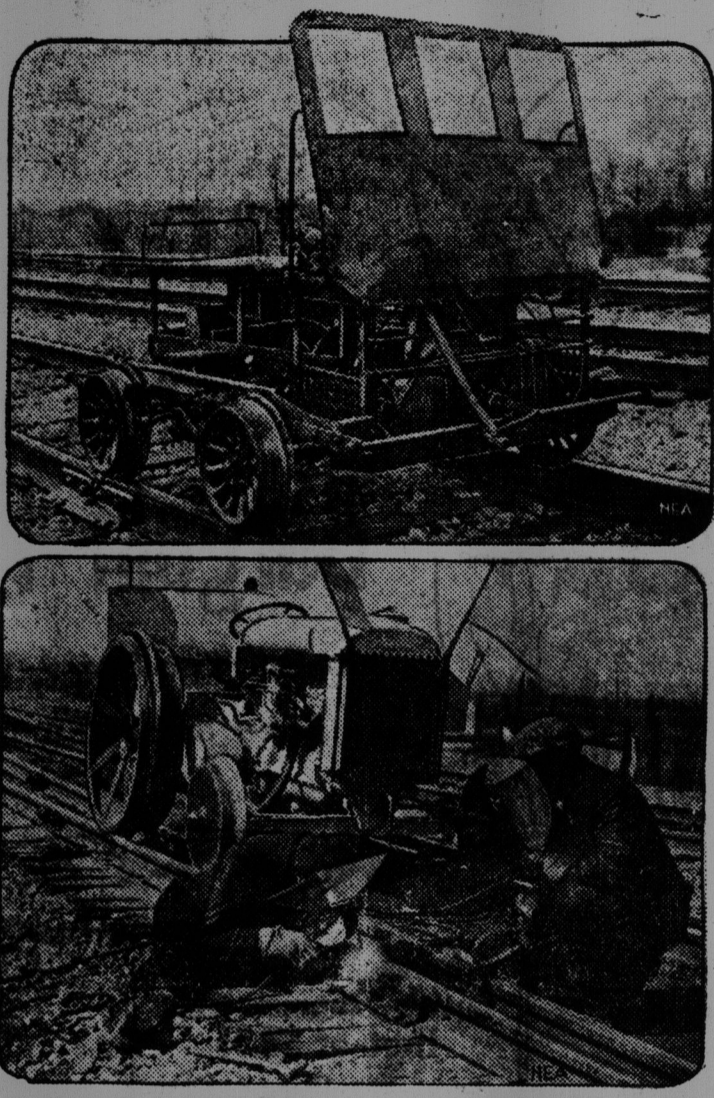
Henry Ford's Detroit, Toledo & Ironton railroad is rapidly becoming flivverized. These photos show two innovations that smack of the automobile industry rather than of the railways. Above is one of the road's hand-cars all fixed up with a windshield; below is a picture of a couple of track repairers who use a Ford tractor, with flanged wheels, to go up and down the track.
