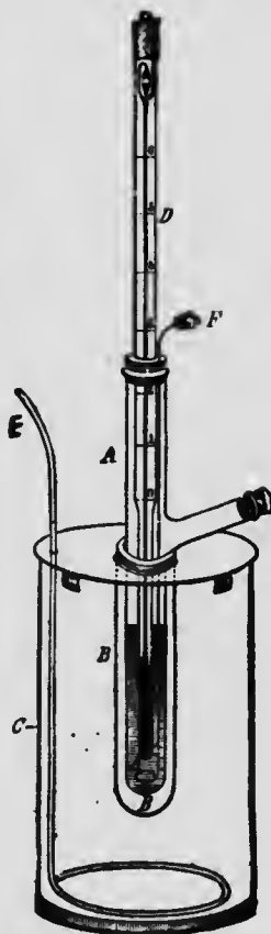
FIG. 14.—BECKMANN'S CRYOSCOPE.
