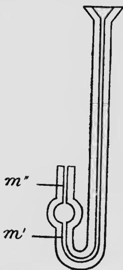
FIG. 13.—VISCOSIMETER OF DENNING AND WATSON.
