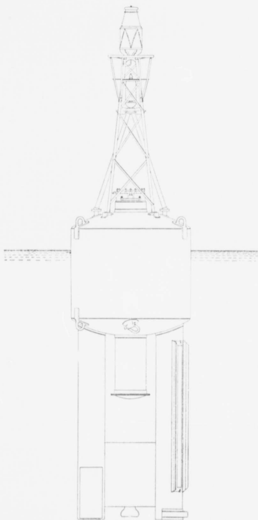
Automatic Whistling and Acetylene Buoy.
