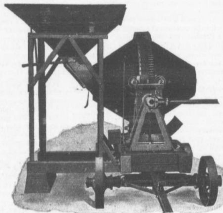
Smith Concrete Mixer with Batch Feeding Hopper
