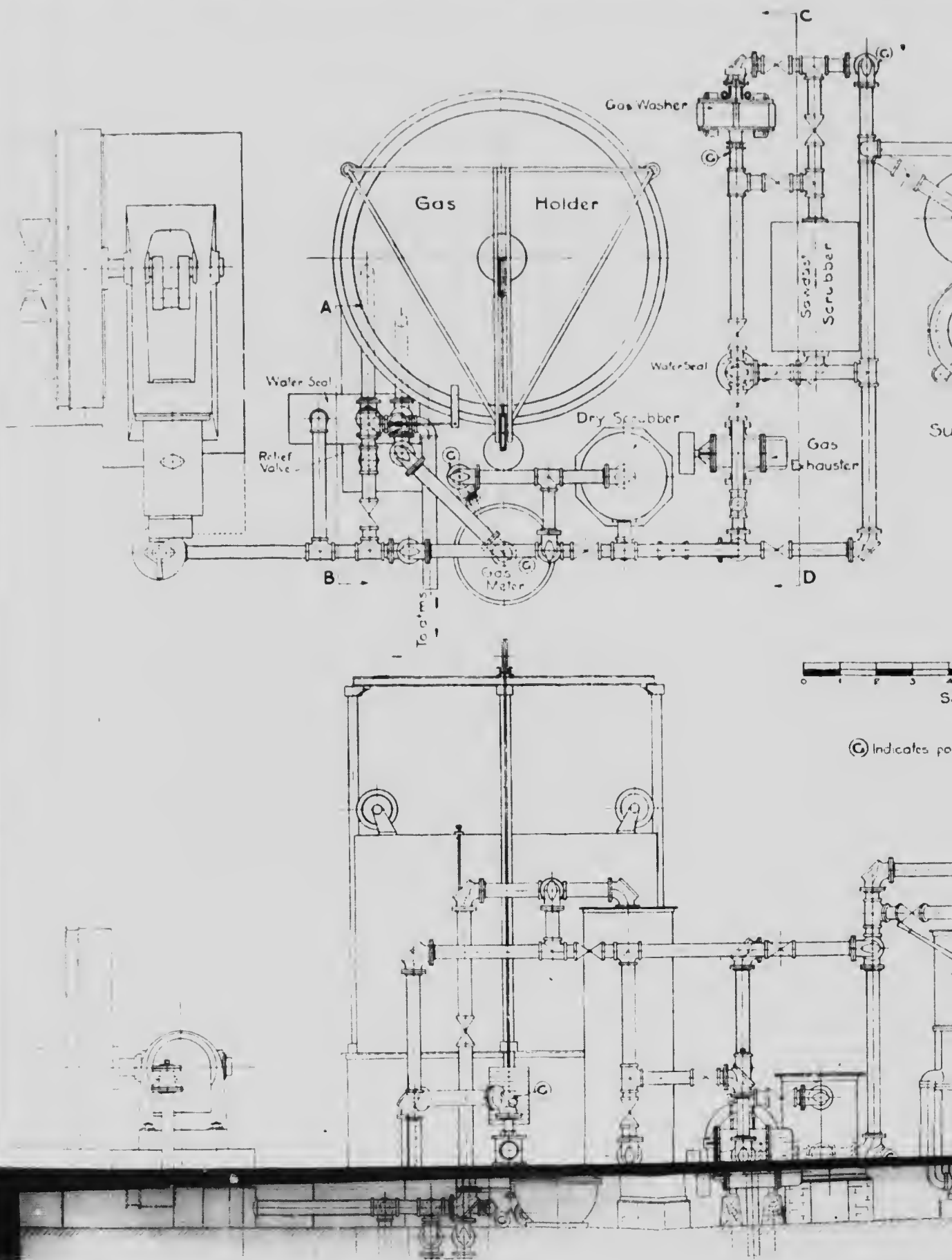
Fig. 18. General arrangement of experimental producer gas plant.
