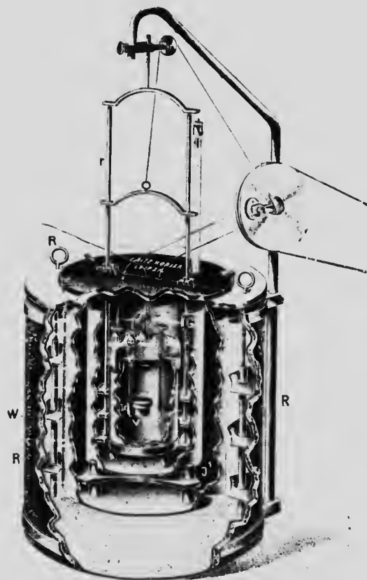
Fig. 52. Vertical section, Koehler calorimeter.
