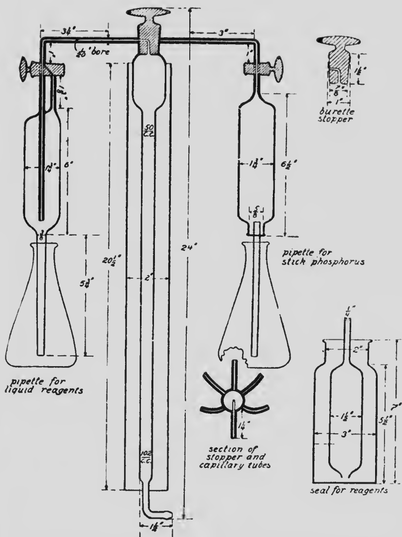
Fig. 53 Section of glass parts of Randall and Barnhart gas analyzing apparatus.
