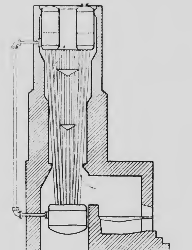
Cahill water tube boiler.
