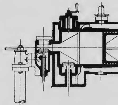
Fig. 46. Forty horse-power gas engine. Department of Mechanical.
