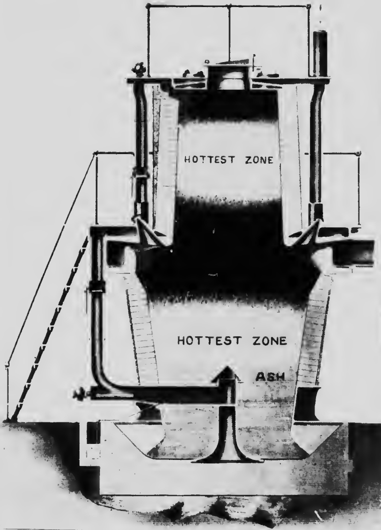
Diagram of Westinghouse double zone producer - vertical section.
