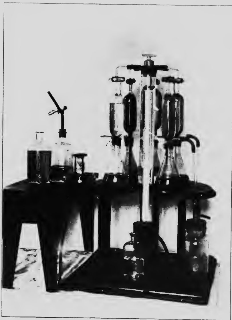
Randall and Baruchart gas analysing apparatus: general view. Department of Mining and Ore Dressing, McGill University.
