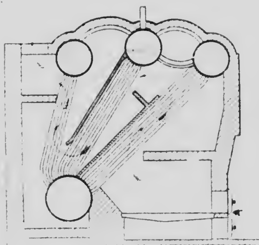
Stirling water tube boiler.
