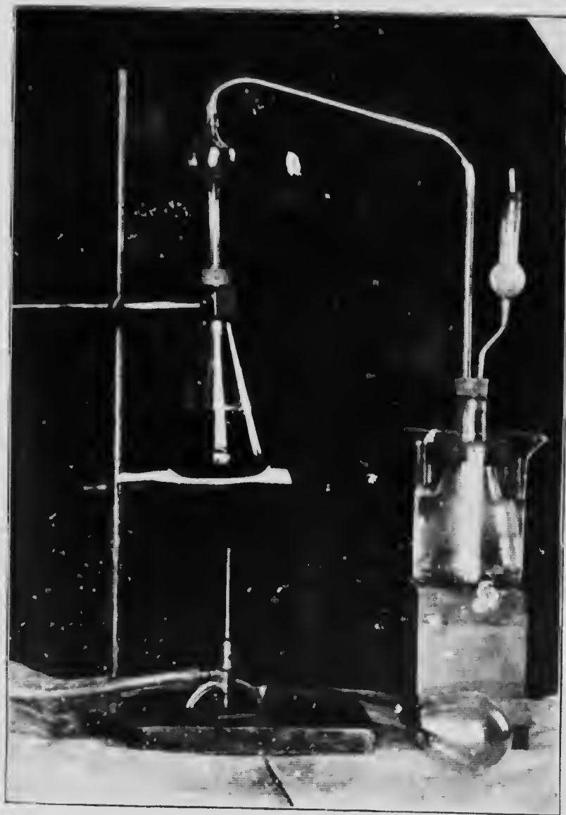
Refrigerated nitrogen distillation apparatus, Chemical Laboratory, Department of Mining and Ore Dressing, McGill University.
