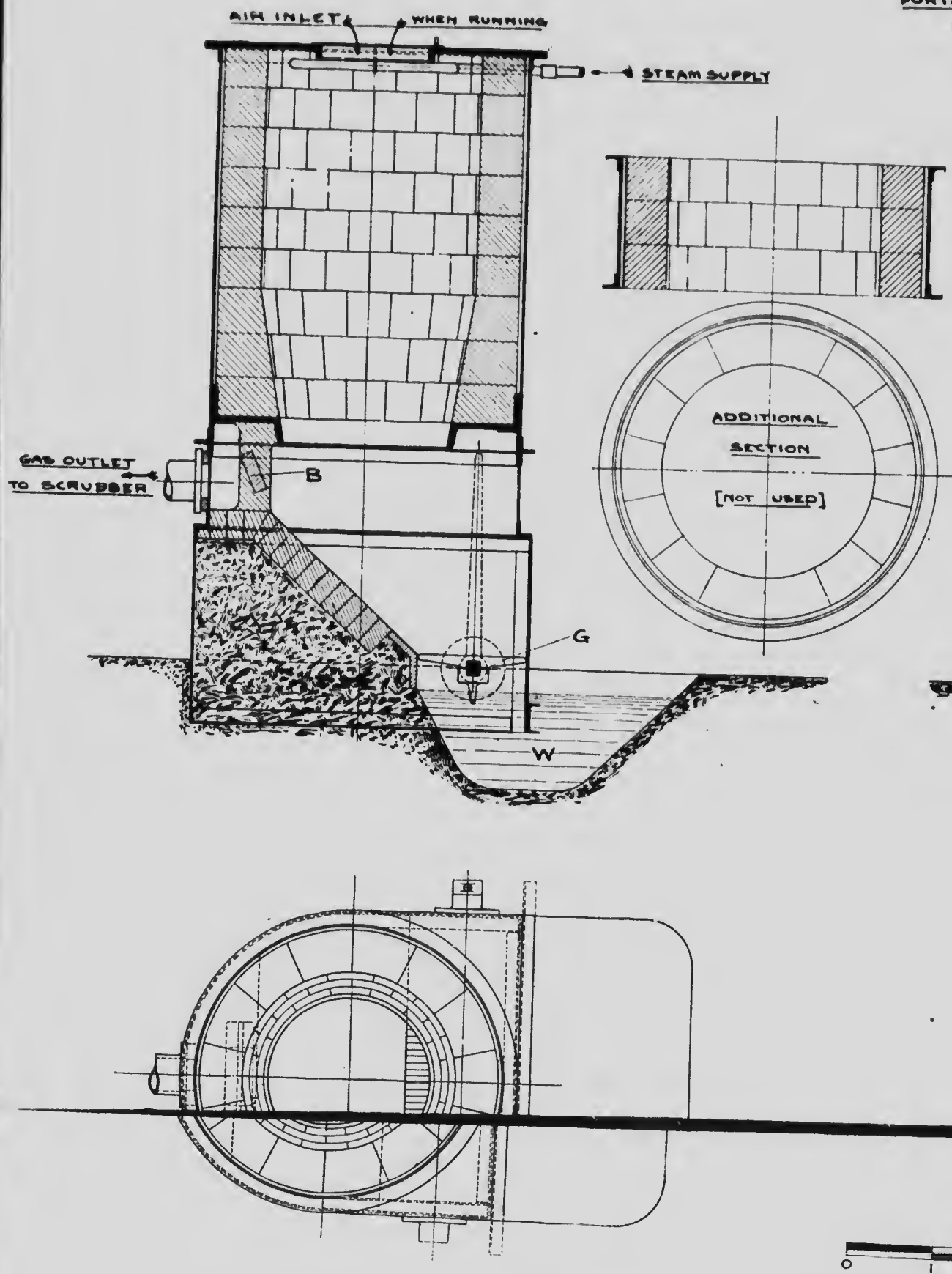
Fig. 45. Down-draft producer, No. 4. Department of Mechanical Engineering
