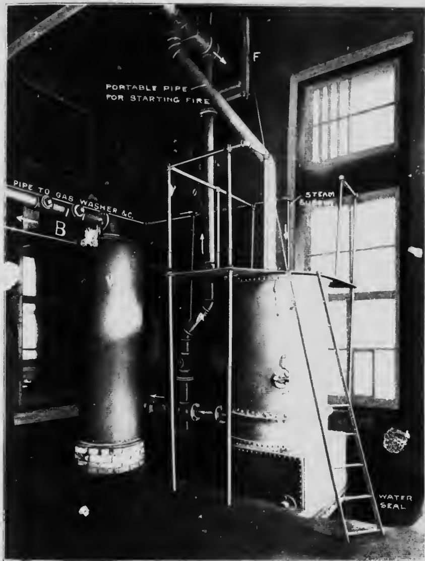
Down-draft producer (No. 1). Department of Mechanical Engineering, McGill University.
