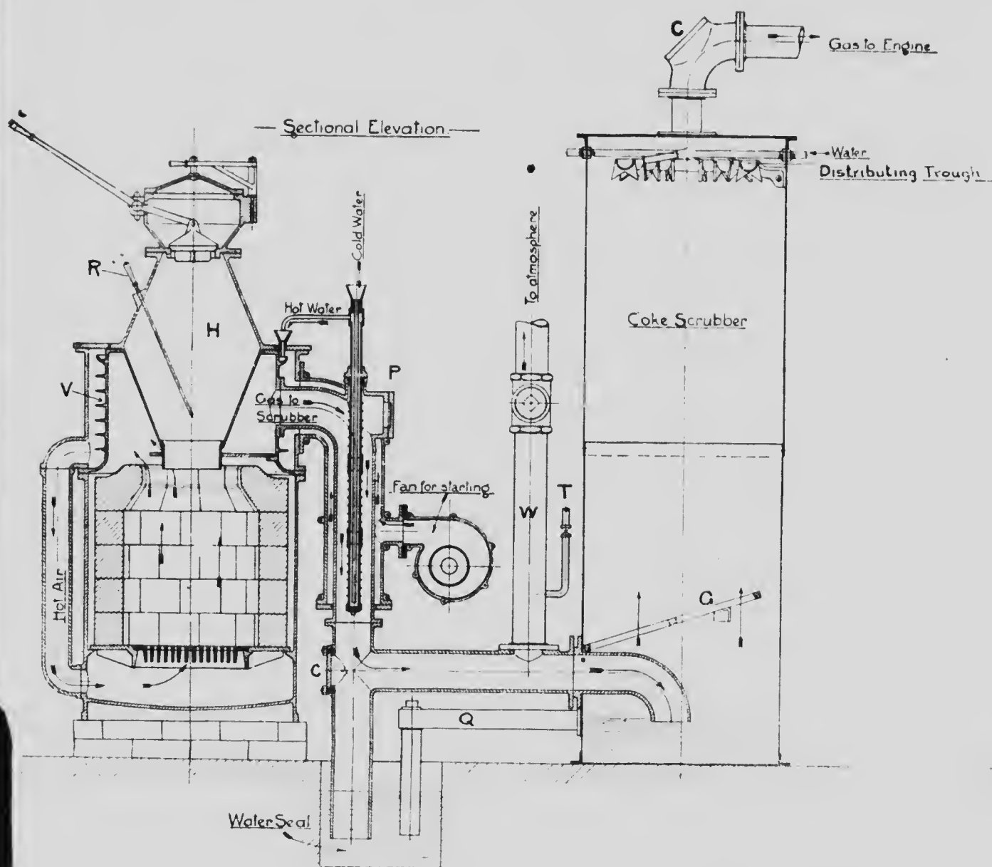
Fig. 44. Suction producer (No. 1). Department of Mech.
