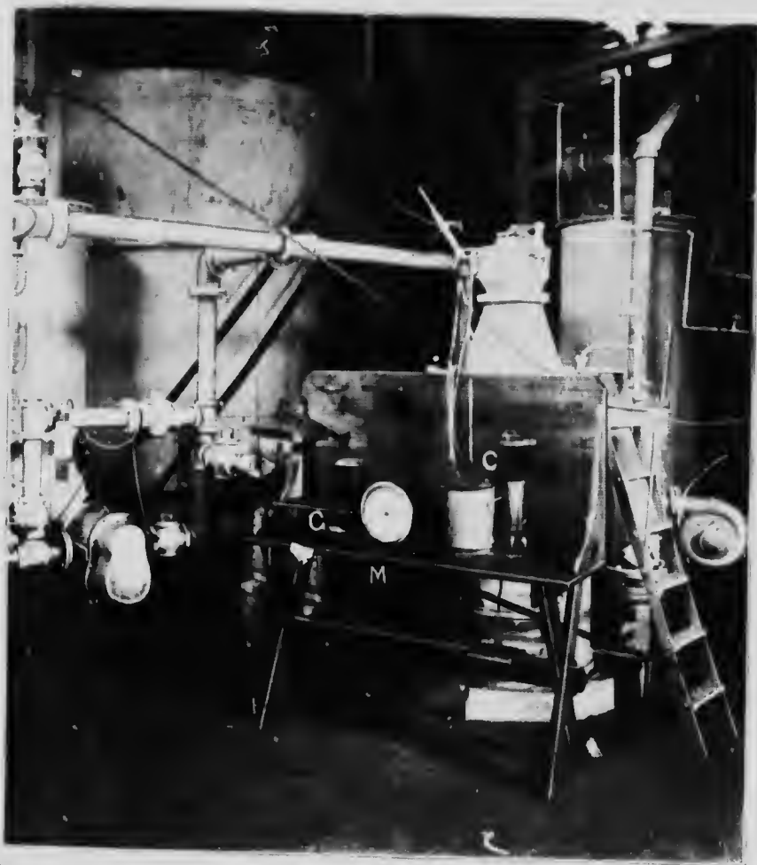
Boys gas calorimeter as set up for producer tests. Department of Mechanical Engineering, McGill University.
