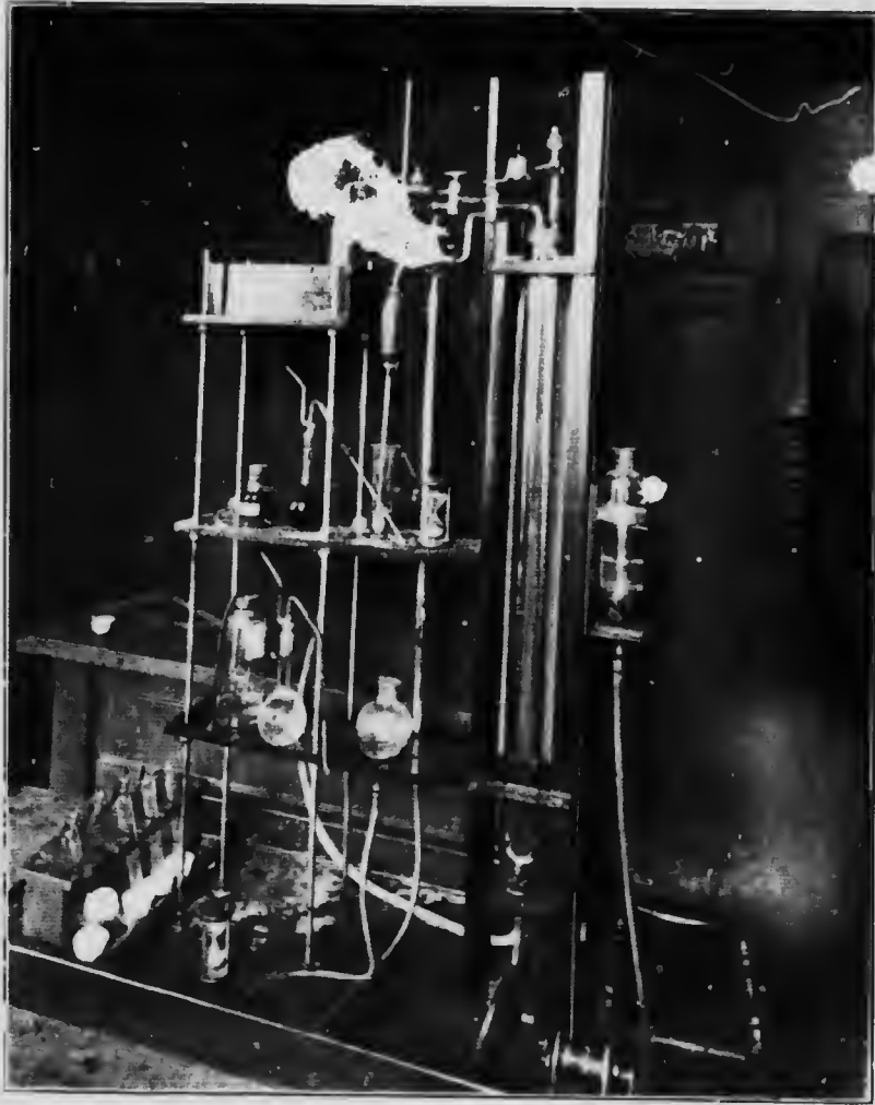
Bone and Wheeler gas analysing apparatus: general view. Department of Mining and Ore Dressing, McGill University.
