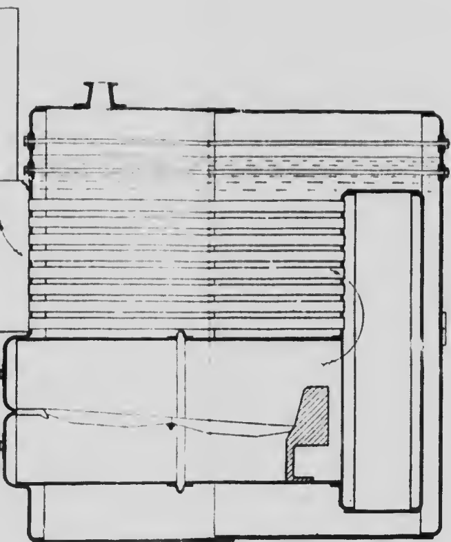
(c) Section of marine boiler.
