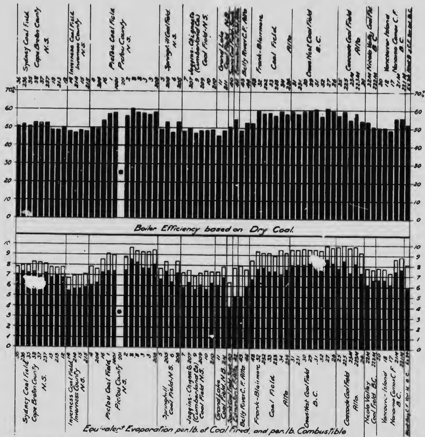
Fig. 37. Diagram showing boiler efficiency and equivalent evaporation.
