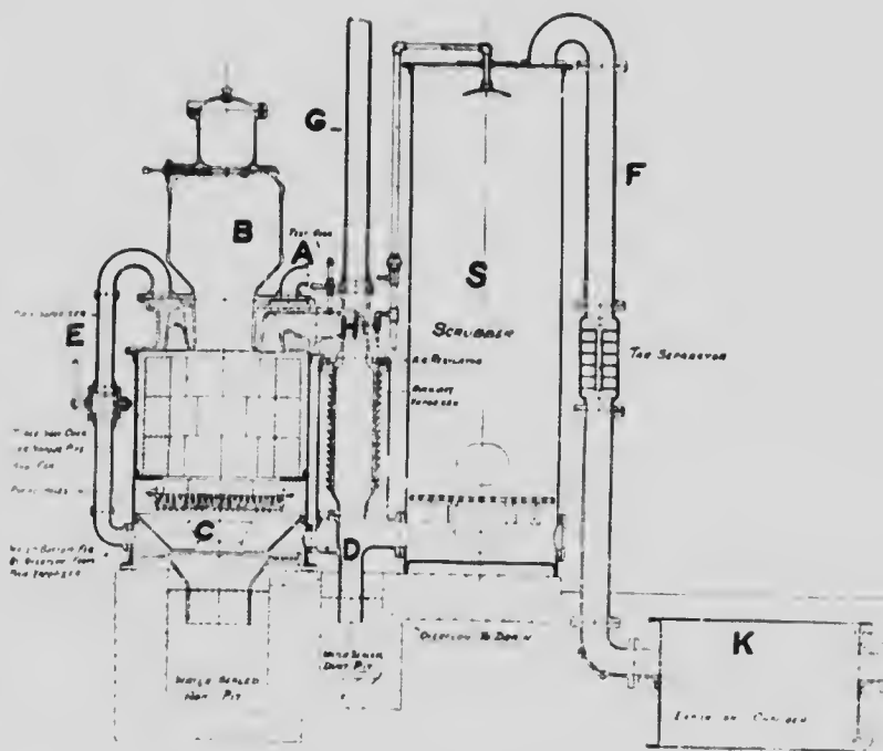
Fig. 29. Suction gas producer. (U.S. Pat. 1,010,100, 1911, L. C. Eng.)
