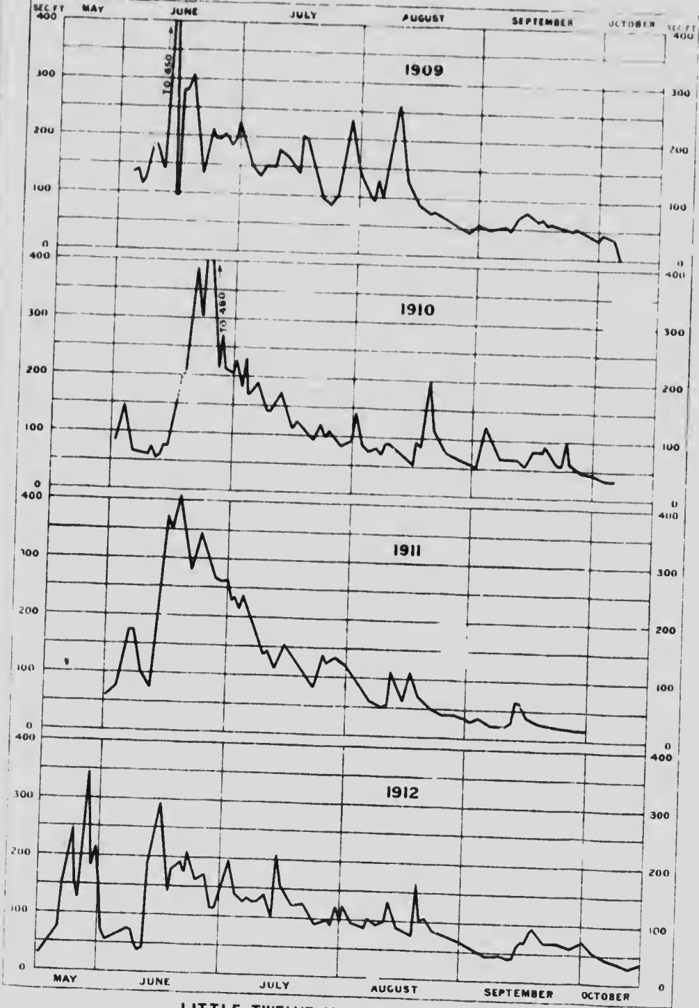
LITTLE TWELVE-MILE RIVER, YUKON HYDROGRAPHS FOR SEASONS 1909-12
