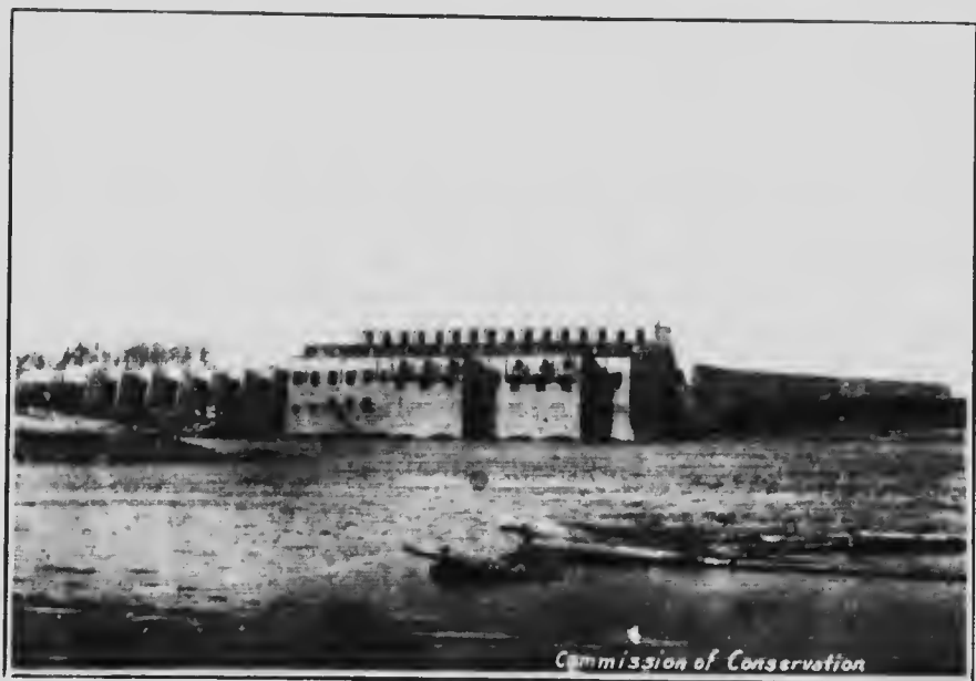
RIVIERE WINNIPEG. USINE HYDRO-ELECTRIQUE MUNICIPALE DE WINNIPEG A POINTE DE BOIS
