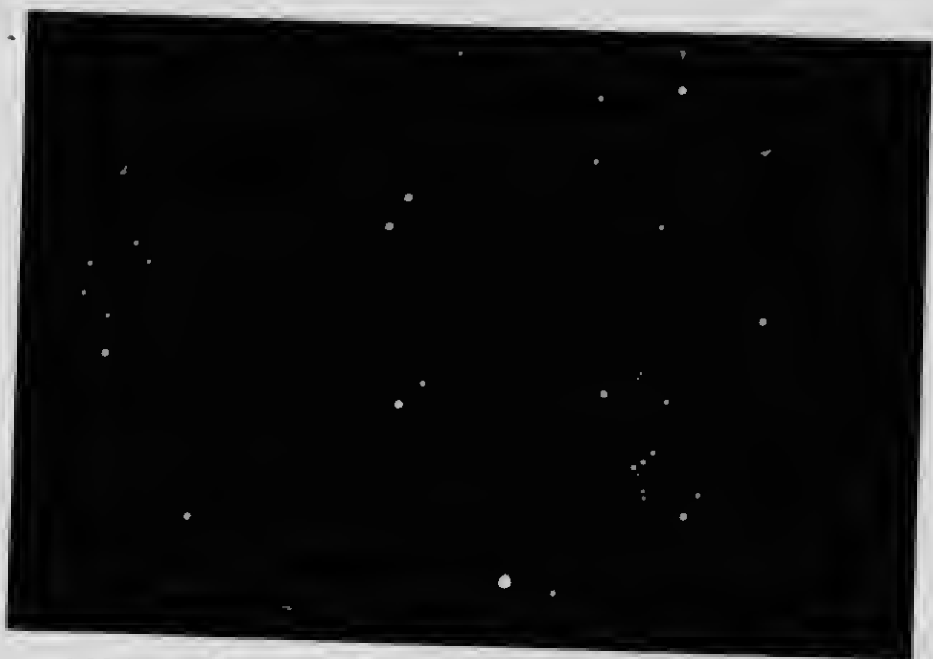
GRO'S CHART OF THE STARS AS HE CALCULATED THAT THEY WOULD APPEAR AT HIS AWAKENING
