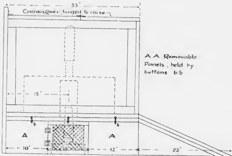
Cut 2. End elevation of brooder. Note sloping run to floor, hinged cover, removable side panel A A on base of brooder. In the centre of this is a small door made of \frac{1}{4} inch mesh galvanized wire. Through this door the lamp is withdrawn for filling and cleaning. The panel A A is removed from the brooder, is dismantled, and the whole superstructure is then packed away under the base. See text for further explanation.
