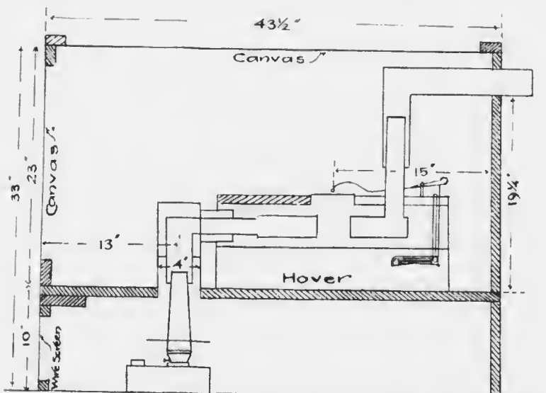
Cut 3. Section through middle of brooder. Note cloth cover and slide, large space between floor of brooder and floor of house, in which the lamp is placed while the brooder is in operation, and which serves as a storage place for the whole upper part of the brooder when the latter is not in use.
