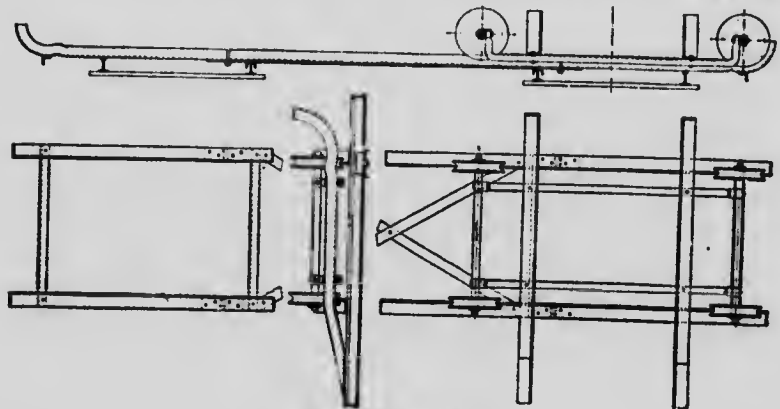
Fig. 111. Chariot.
