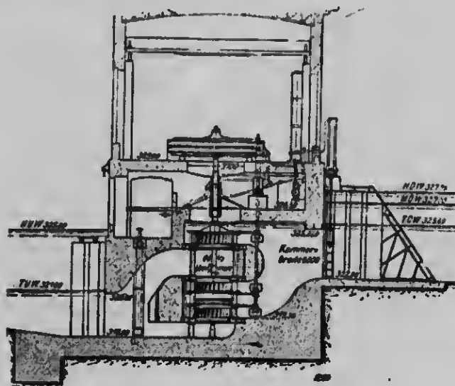
Fig. 6.—Beznav: Section through unit.
