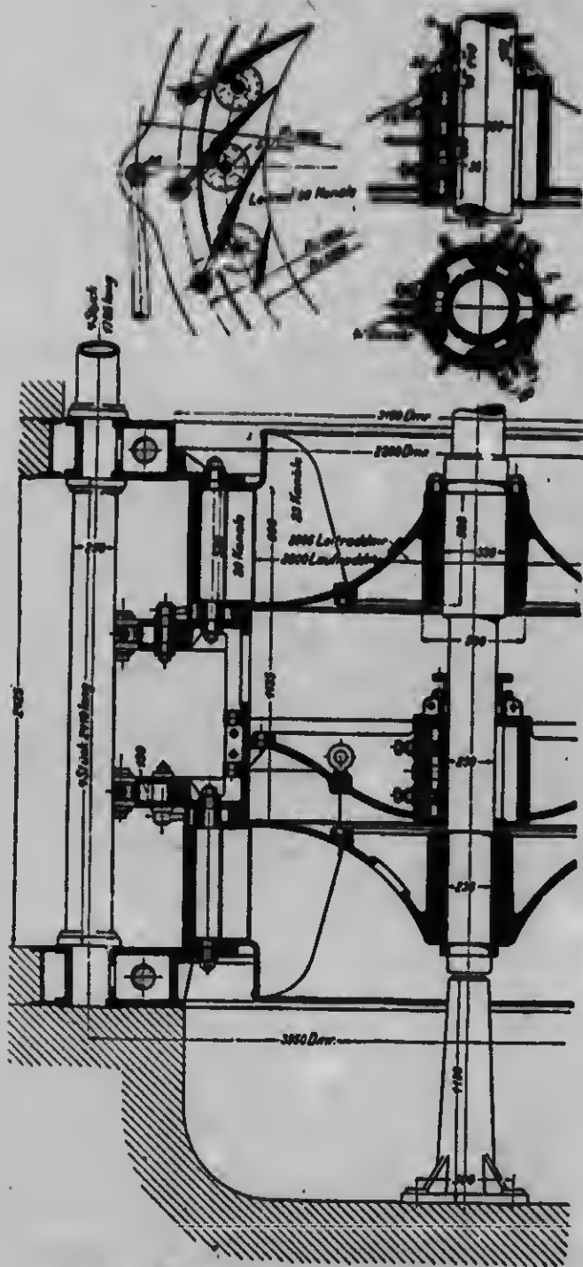
Fig. 7. Bernau. Details of Turbine Unit.
