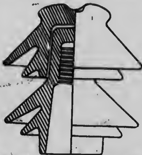
Fig. 5.—Paderno: Standard Line Insulator.
