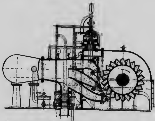
Fig. 4.—Kubei: Section Through 1,200 H. P. Wheel.
