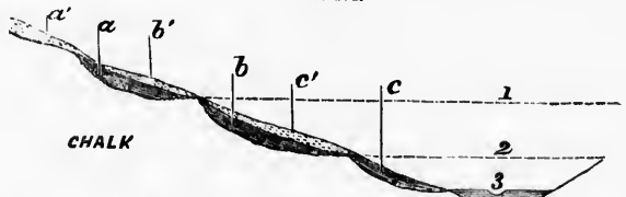
Diagram to show the Relations of the Loëss and the Gravels.
