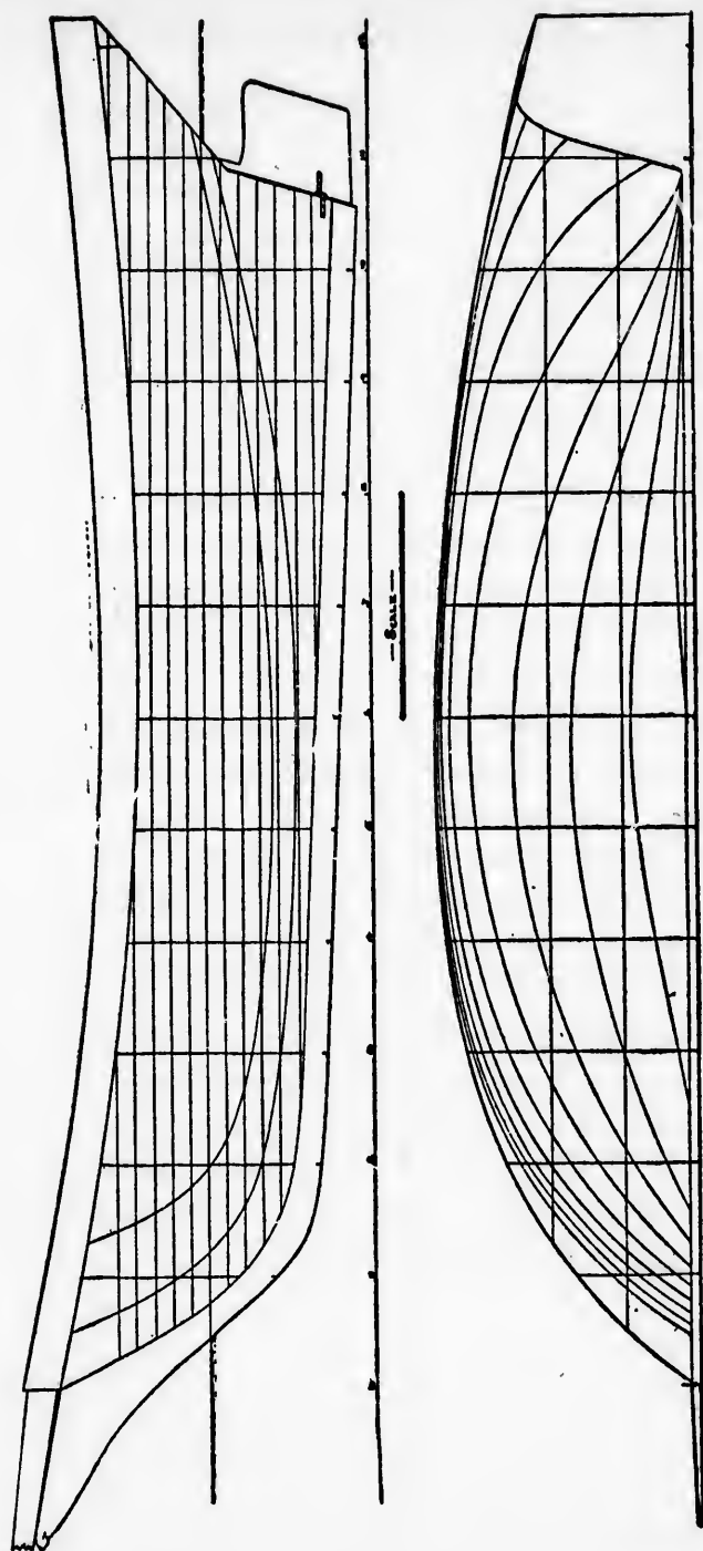
Lines of the Spray .
