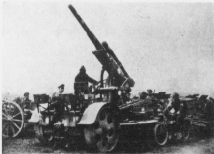
AN ANTI-AIRCRAFT GUN CAPTURED BY THE CANADIANS.
