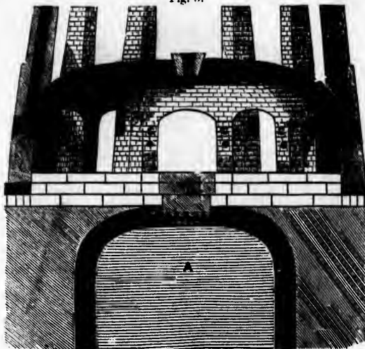
Section of Elevation.—A, Air Tunnel below the Furnace. B, Pit of Furnace, with Grates below. C, Flue Holes, through which the Flame passes to the Flues above.
