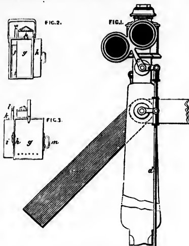
Boake's Irish Railway Signal Post.
