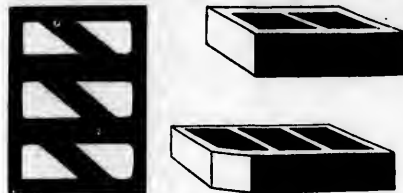
Sections of the Hollow Bricks of the Model Structure.
