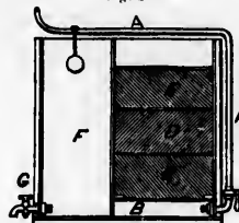
Stirling's Patent Slate Filters.
