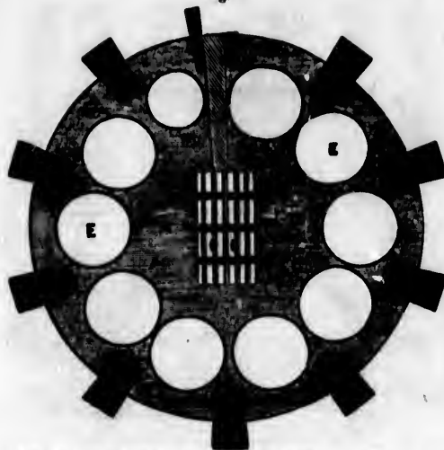
Ground Plan.—AA, "Sieve" or Floor of Furnace. BB, Pillars, which support the Crown. CC, Grates. D, Furnace Door. E, Position of Crucibles.
