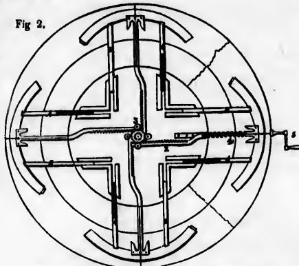
Hawkins's Patent Cog-wheel Movement for Dining-tables.
