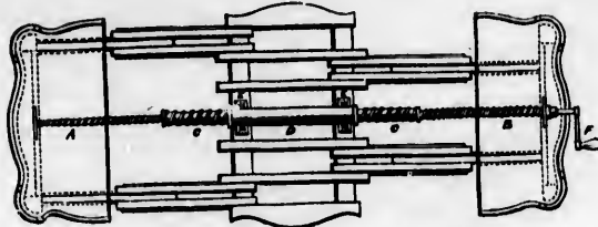
Hawkins's Patent Screw Movement for Dining-tables.
