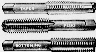
Set of Hand Taps.
