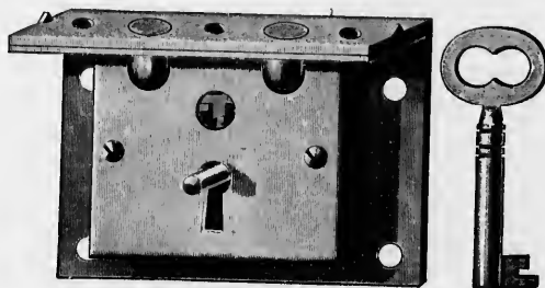
No. 427—2½ inch, IRON, square seldge, solid square box, screwed, 2 secure levers, double link, fine flat bow keys, all different in a dozen.....Per dozen $3.00
