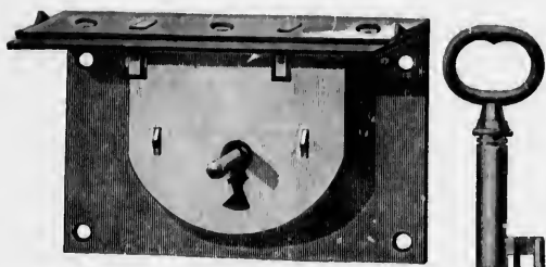
No. 166—2½ inch, Iron, double link, 1 ward, four changes in a dozen..... Per dozen $2.12 Corresponding numbers, Yale S1, Corbin 34. One dozen in a box.
