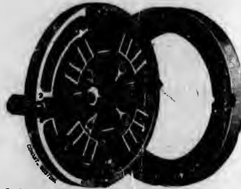
Inside view of 1 1/2 inch Four Jaw Chuck, showing the Screws and Pinions, the Nut under the Jaw, and the Gear which is loose in the Back Shell.
