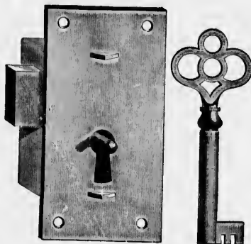
No. 416— 2\frac{1}{2} x 1\frac{1}{2} inch (brass), solid square box, tumbler, bolt shoots right and left. Per dozen ..... $2.00 Corresponding numbers, Yale WA3, Corbin, 0702.
