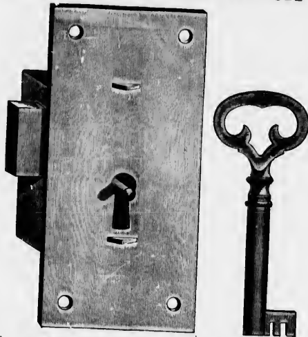
No. 392— 3\frac{1}{2} x 1\frac{1}{4} inch, iron, solid square box, broad bolt, shoots right and left, tumbler..... Per dozen 81.75 Corresponding numbers, Yale W14. Corbin 710.
