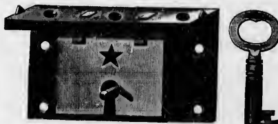
No. 585—2 inch, ALL BRASS, square seldge, solid square box, 1 secure lever, double link, fine flat bow keys, four changes in a dozen.....Per dozen $3.00
