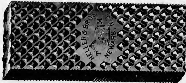
Exact width, thickness and appearance of centre section of 16 inch Horse Rasp.
