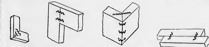
Fig. 8 shows the Fastener applied to prevent splitting at a mortise. When so applied to the rims of wheels, it positively prevents splitting out from the spoke tenons.
