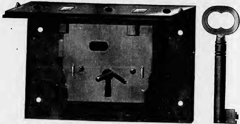
No. 202—4 inch, Iron, double link, 2 secure levers, screwed, fine flat bow keys, all different in a dozen. Per dozen $19 Corresponding numbers, Yale S77, Corbin 72. One dozen in a box.
