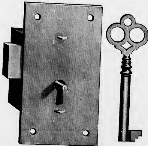
No. 174— 3\frac{1}{2} x 2 inch, iron, solid square box, broad bolt, shoots right and left, 2 secure levers, fancy bow keys, six changes in a dozen..... Per dozen 82.25 Corresponding numbers, Yale W52, Corbin 712.
