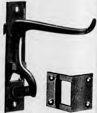
Spiral spring action.
